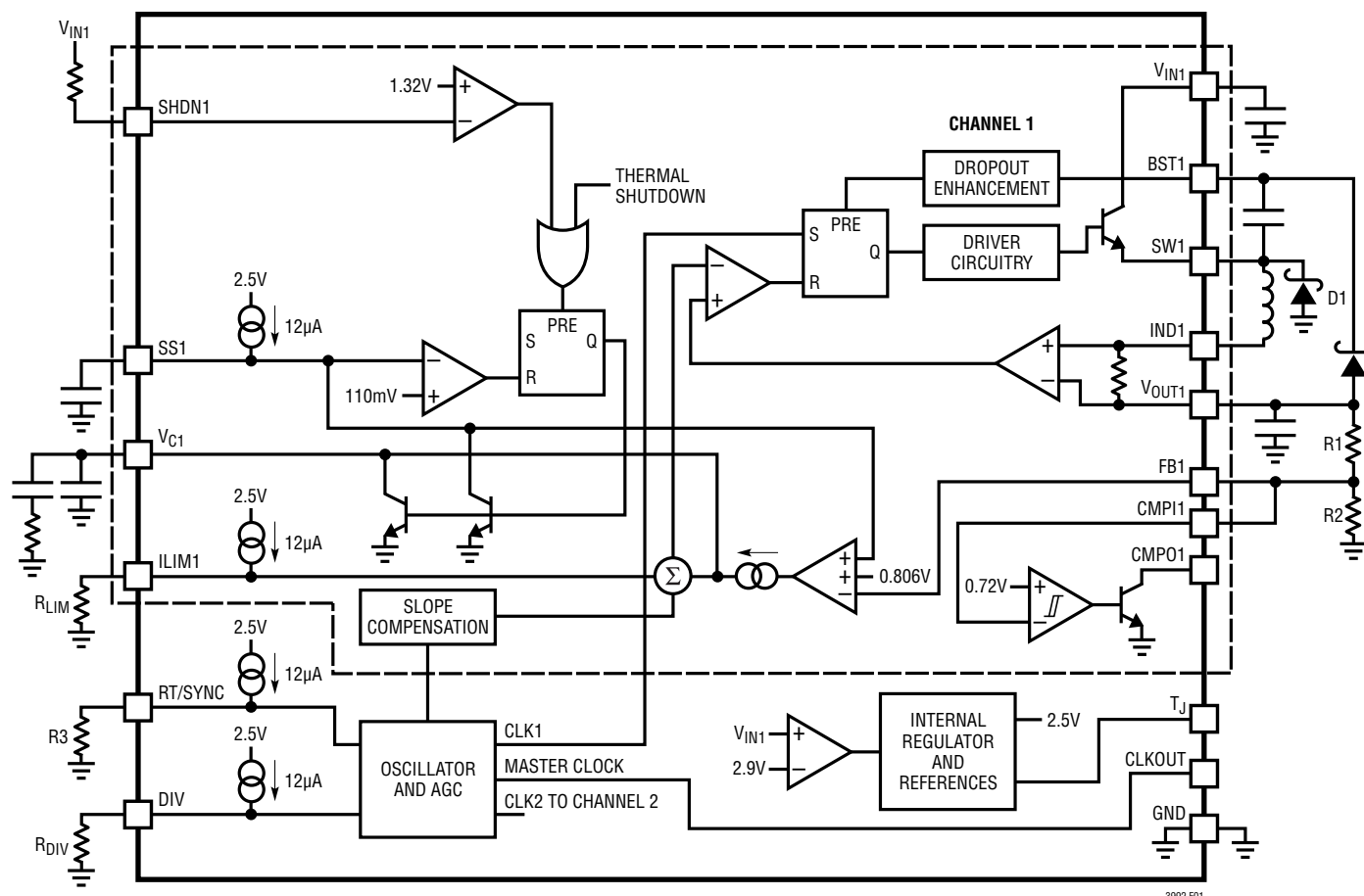
Figure 1. LT3992 Block Diagram
