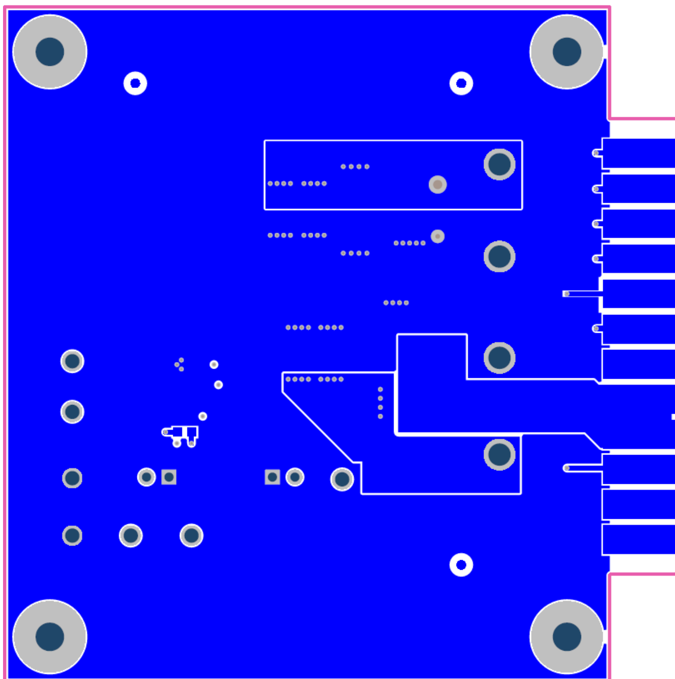
Figure 5. Bottom Layer
