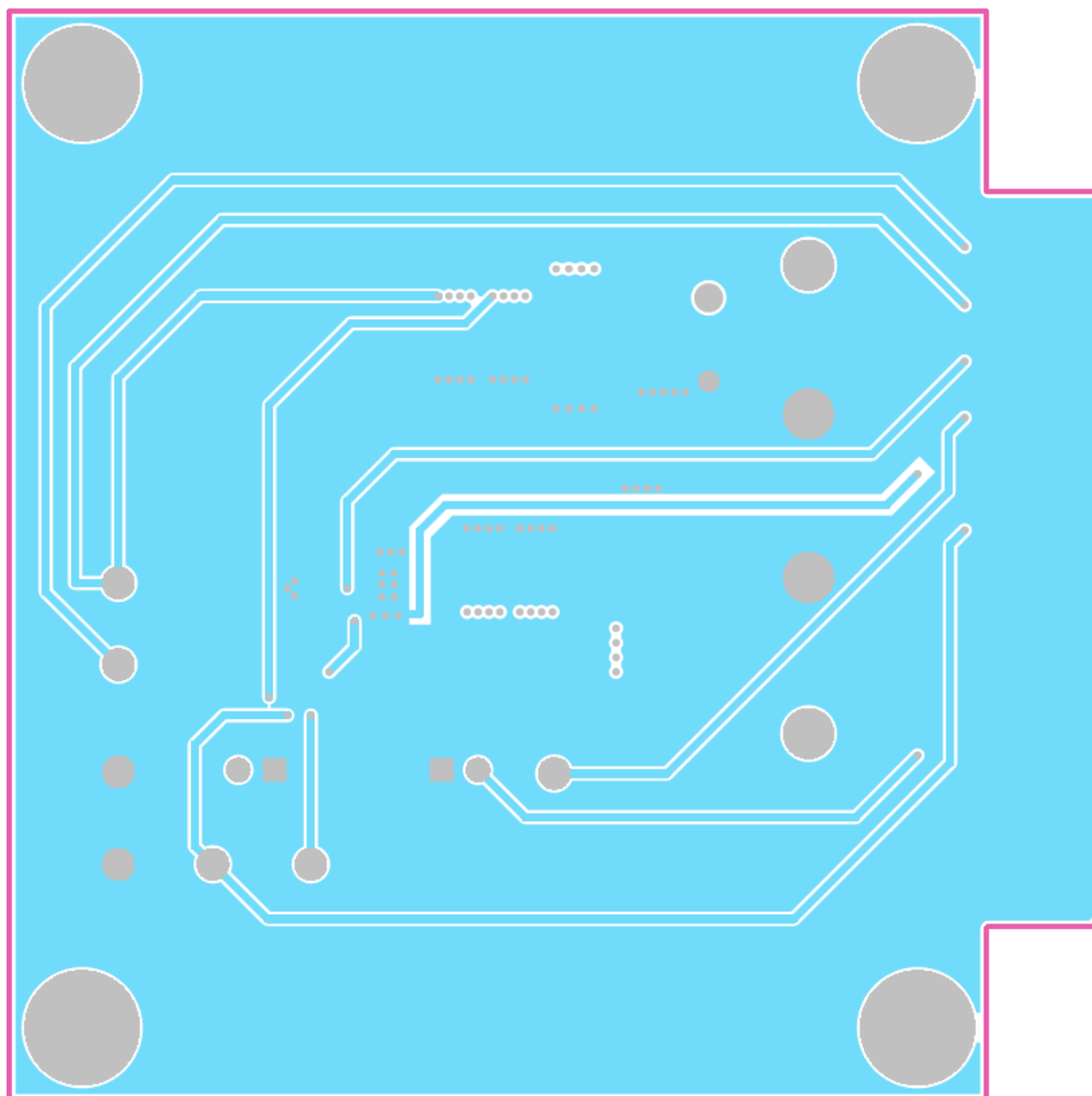
Figure 4. Middle Layer 2
