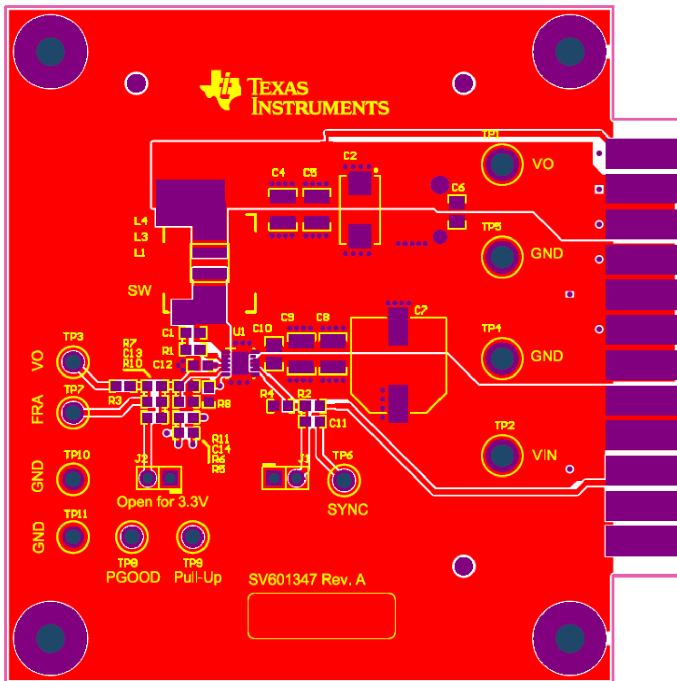
Figure 2. Top Layer
