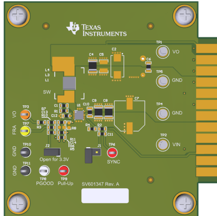
Figure 1. LMR23625CFPEVM Board
