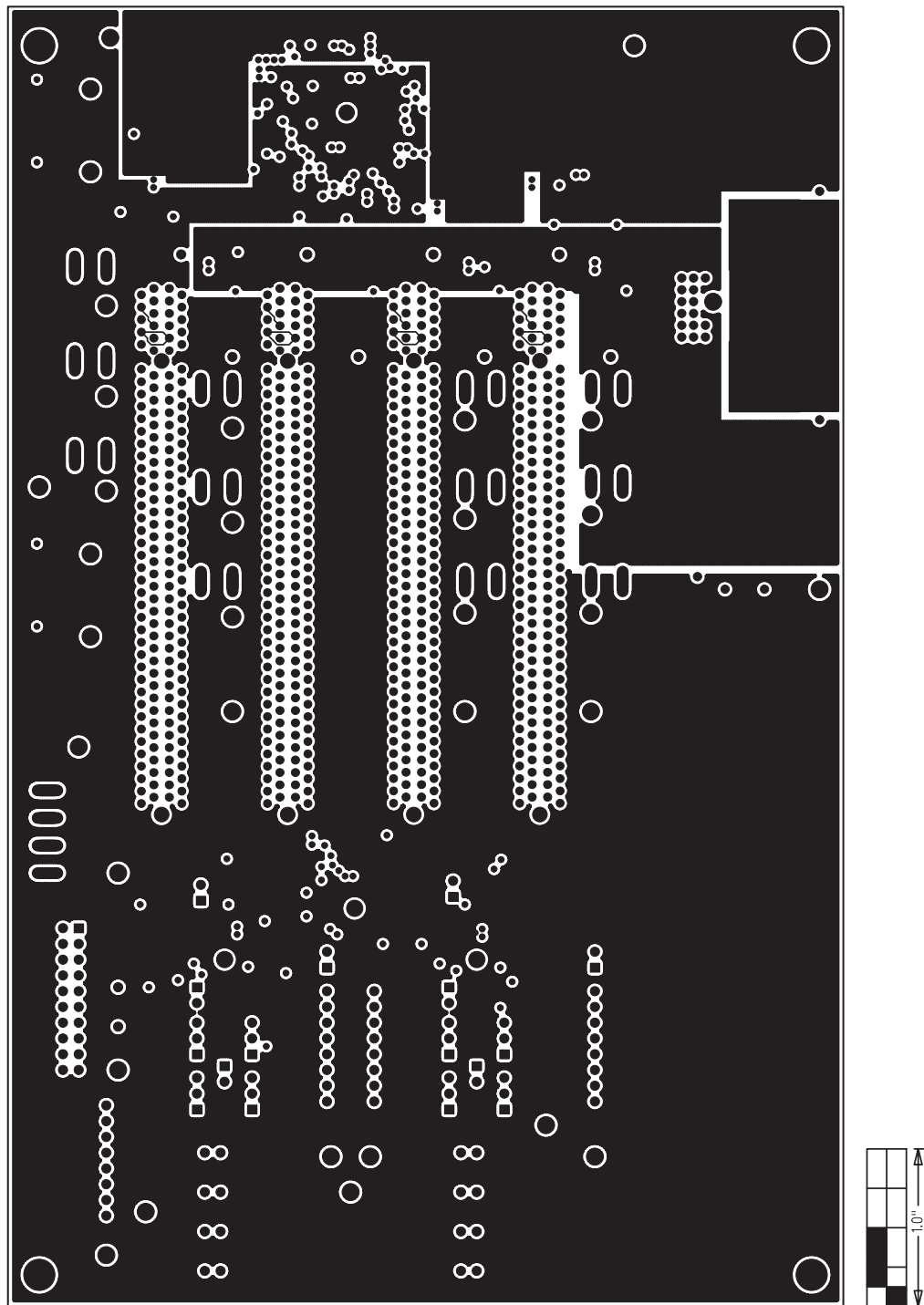
Figure 11. MAX5960L EV Kit PCB Layout—Inner Layer, Power Plane Layer 3
