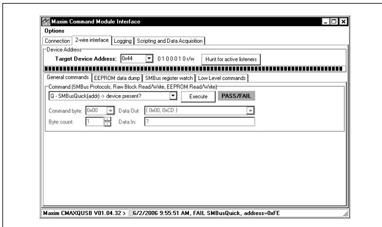
Figure 2. The 2-Wire Interface Window Provides Direct, Low-Level Access to the MAX5960L with the MAX7313 and SMBus 2-Wire Interface
