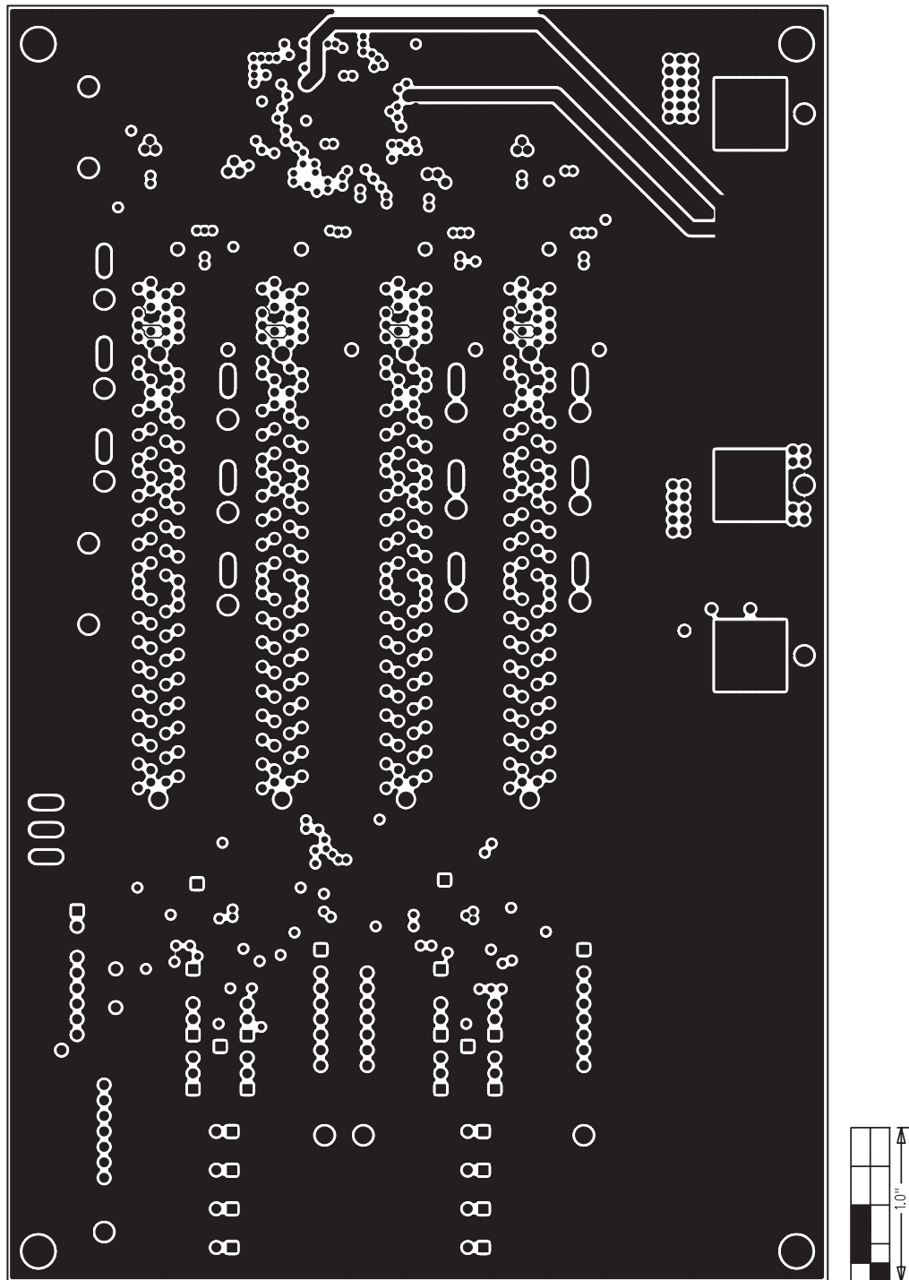
Figure 10. MAX5960L EV Kit PCB Layout—Inner Layer, Ground Plane Layer 2
