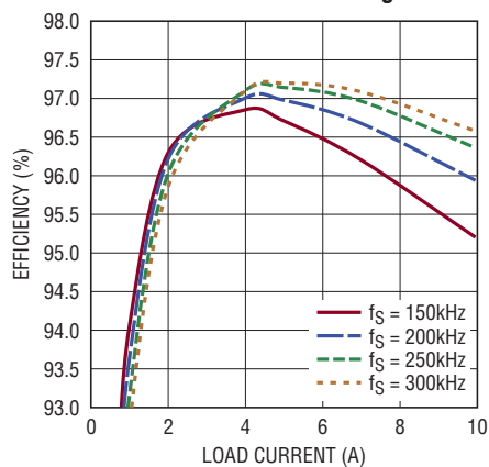
Efficiency vs Load Current 24V to -24V Inverter in Figure 9
