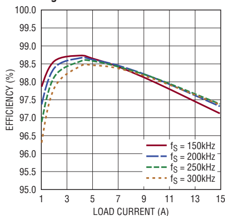
Efficiency vs Load Current 24V to 12V Voltage Divider in Figure 7
