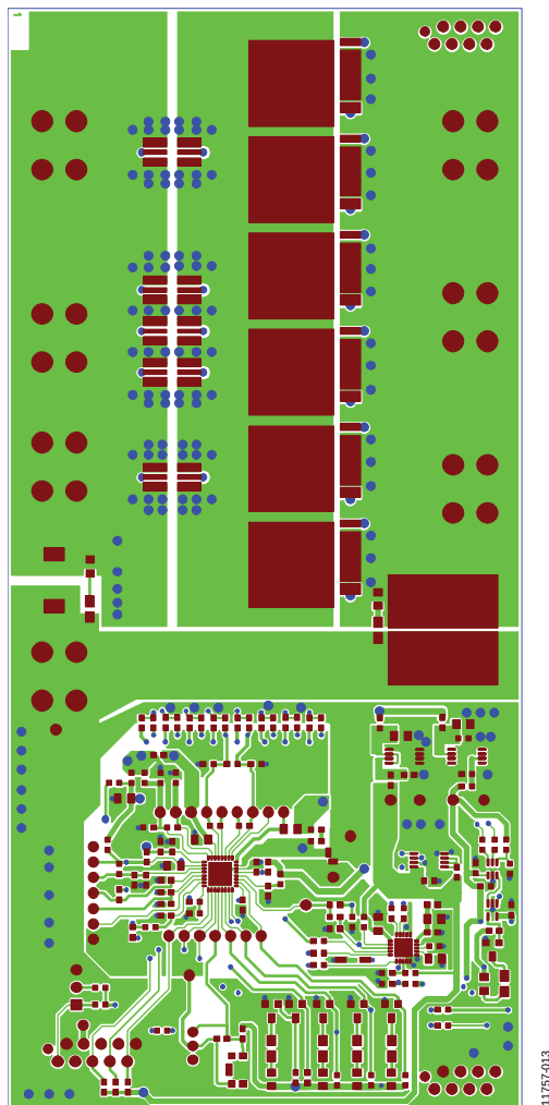
Figure 15. Top Layer 1
