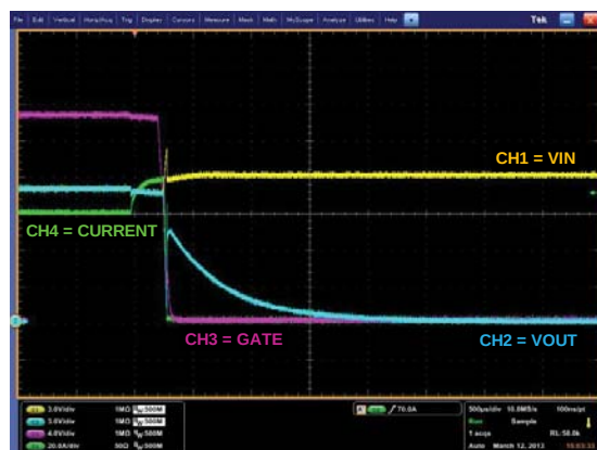
Figure 8. Overcurrent Shutdown
