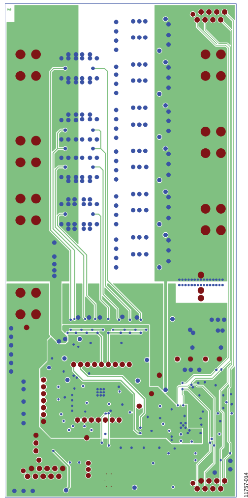
Figure 16. Inner Layer 2
