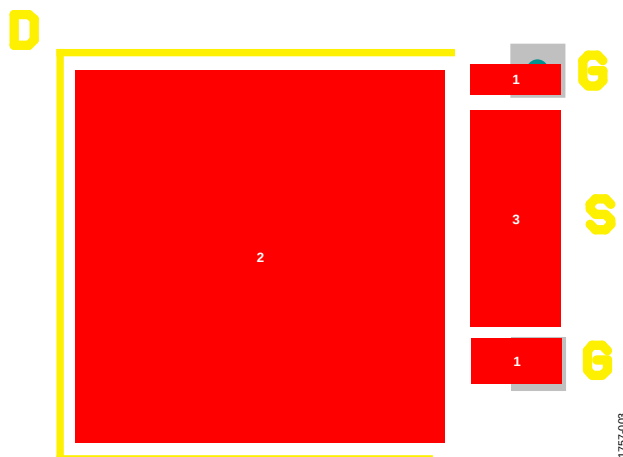
Figure 4. Multipackage N-MOSFET Footprint
