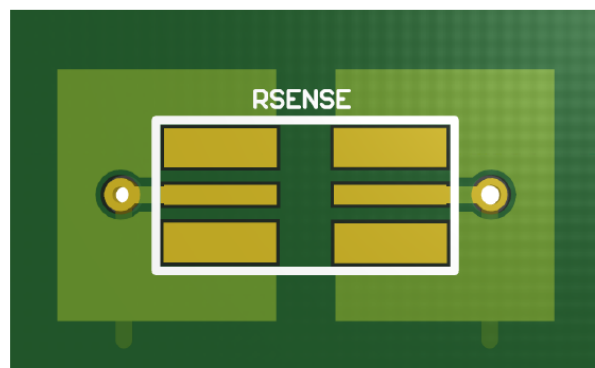
Figure 5. Recommended Sense Resistor Footprint
