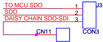
NORMAL OPERATION J3: 1:2 SDO SIGNAL TO MCU DAISY CHAIN J3: 2:3 SDO SIGNAL TO SDI
