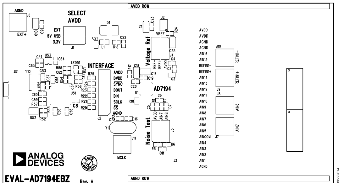
Figure 14. EVAL-AD7194EBZ Silkscreen
