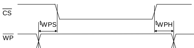
Figure 30. Status Resister Write Timing
