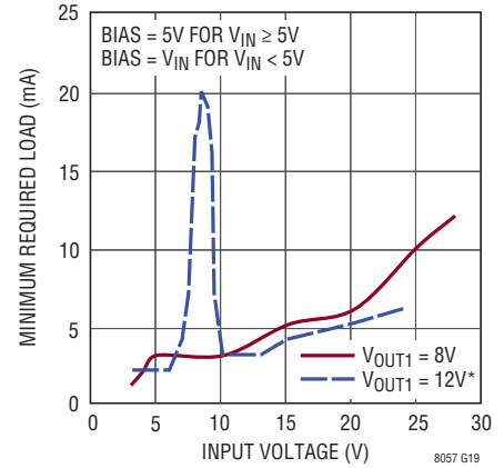
Minimum Required Load vs Input Voltage
