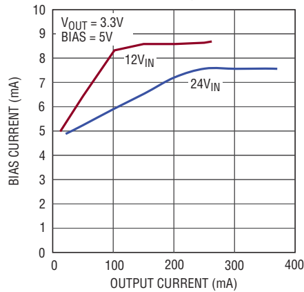
Bias Current vs Output Current
