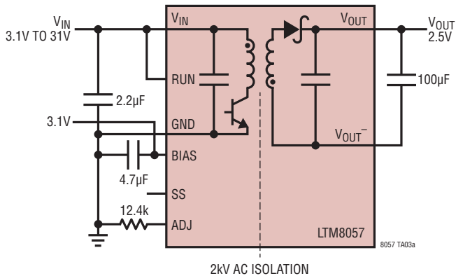
2.5V Flyback Converter
