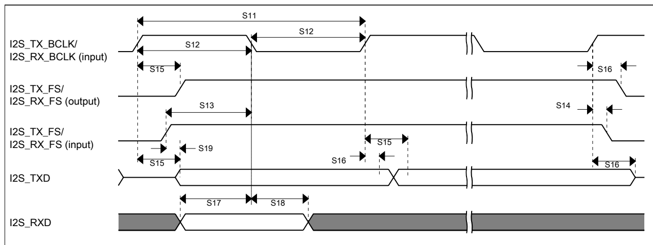
Figure 33. I2S/SAI timing — slave modes
