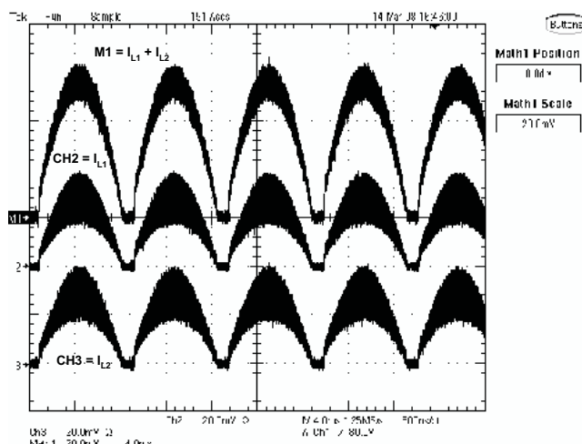
Figure 12. Input and Inductor Ripple Current at V_{IN} = 85 V RMS, P_{OUT} = 300 W
