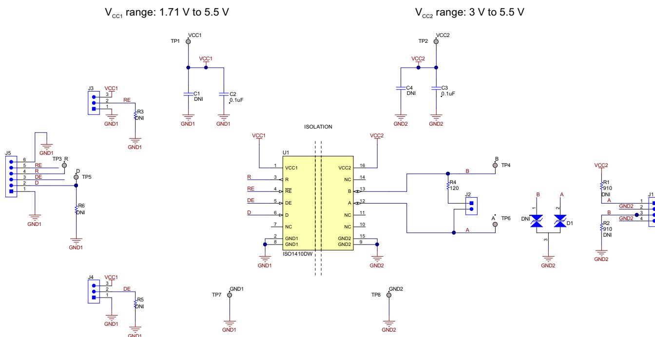
Figure 5. ISO1410DWEVM Schematic
