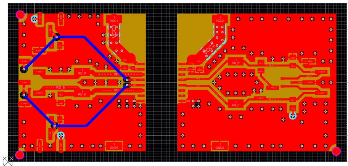
Figure 4. Signal-Layer View Half Duplex Isolated RS-485 EVM
