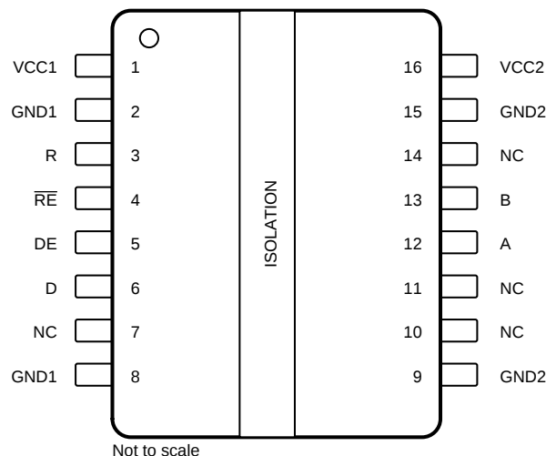
Figure 2. ISO1410 DW Package 16-Pin SOIC Pin Configuration
