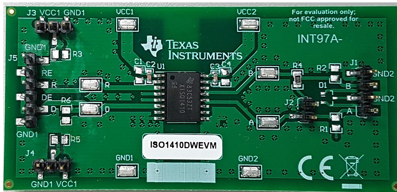
Figure 3. Board Layout
