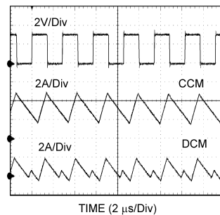
Figure 49. CCM and DCM Operating Modes
