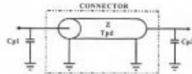
Connector Distributed Model
