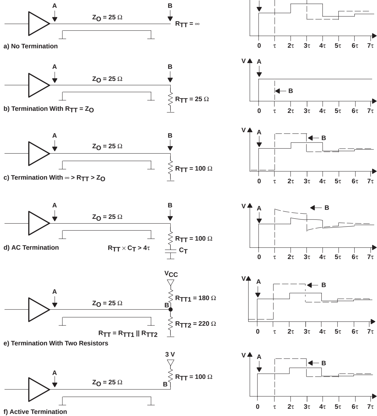
Figure 8. Termination Methods With TTL and CMOS Circuits
