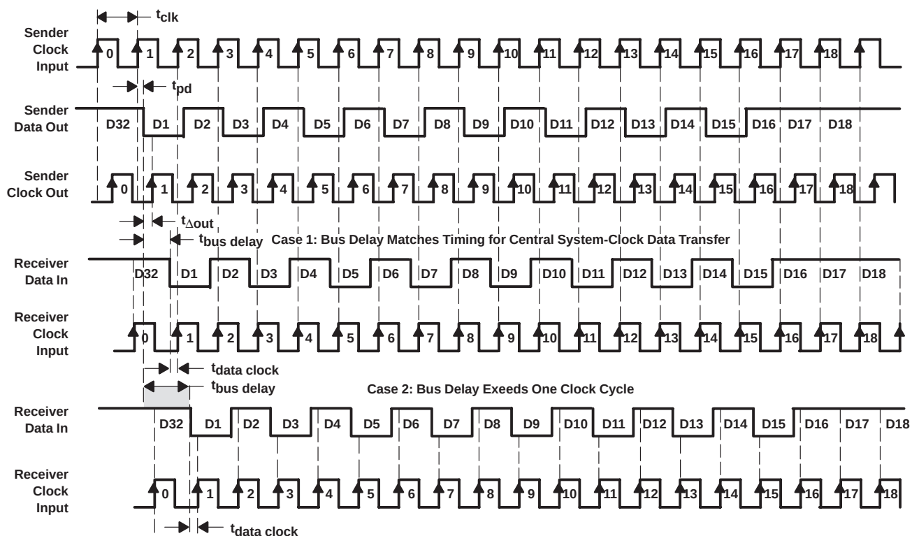
Figure 14. Two Examples of Source-Synchronous Clock Distribution
