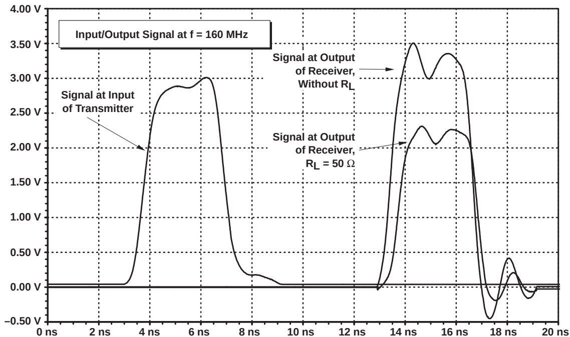
Figure 49. LVTTTL Input and Output Signal of SN74GTLPH1655, ERC = V_{CC} , Loaded, 160 MHz
