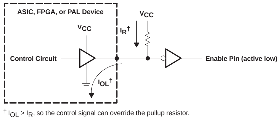
Figure 40. Power-Up High Impedance With Active-Low Control Pin
