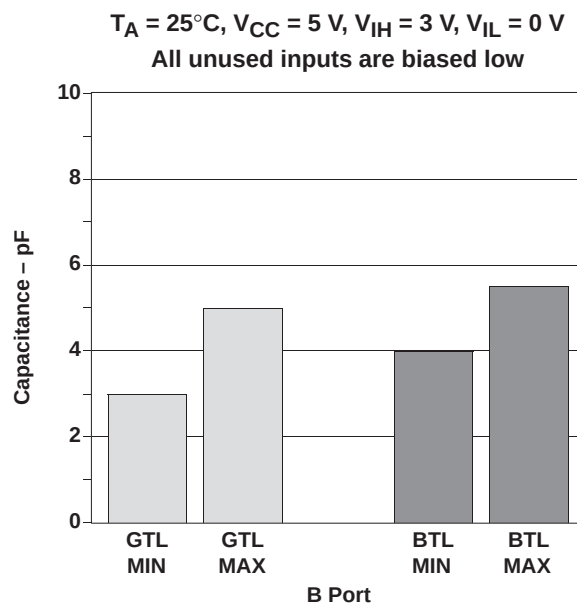
Figure 10. Capacitance Variation Across Process
