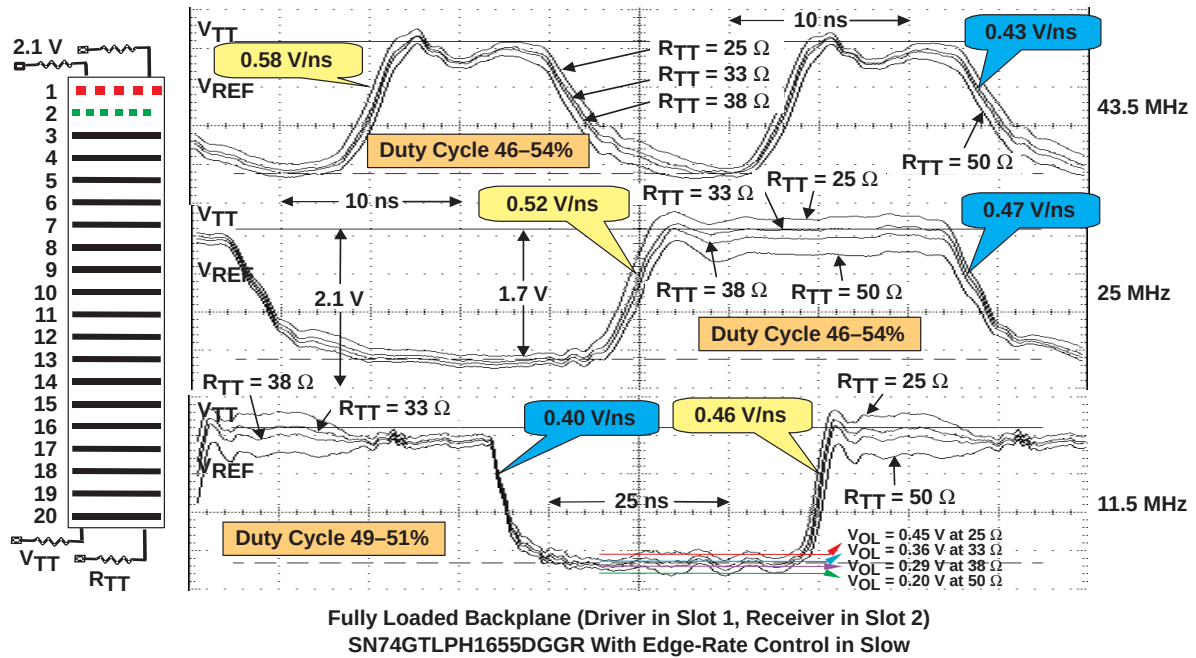
Figure 9. GTLPH1655 Waveforms at BTL Signal Levels (Group 1, Bit 1)
