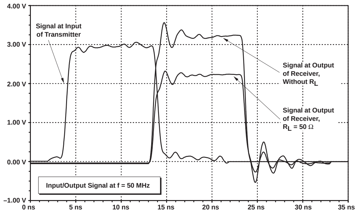
Figure 35. LVTTTL Input and Output Signal of SN74GTLPH1655, ERC = GND, Unloaded, 50 MHz
