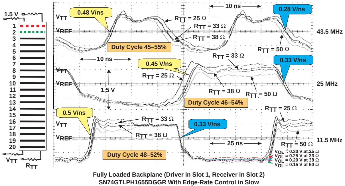
Figure 8. GTLPH1655 Waveforms at GTLP Signal Levels (Group 1, Bit 1)
