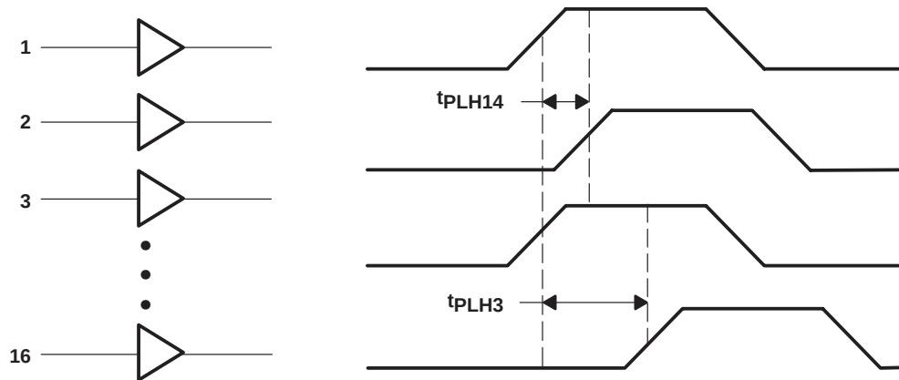
Figure 34. Skew = |t_{PLH3} - t_{PLH4}|
