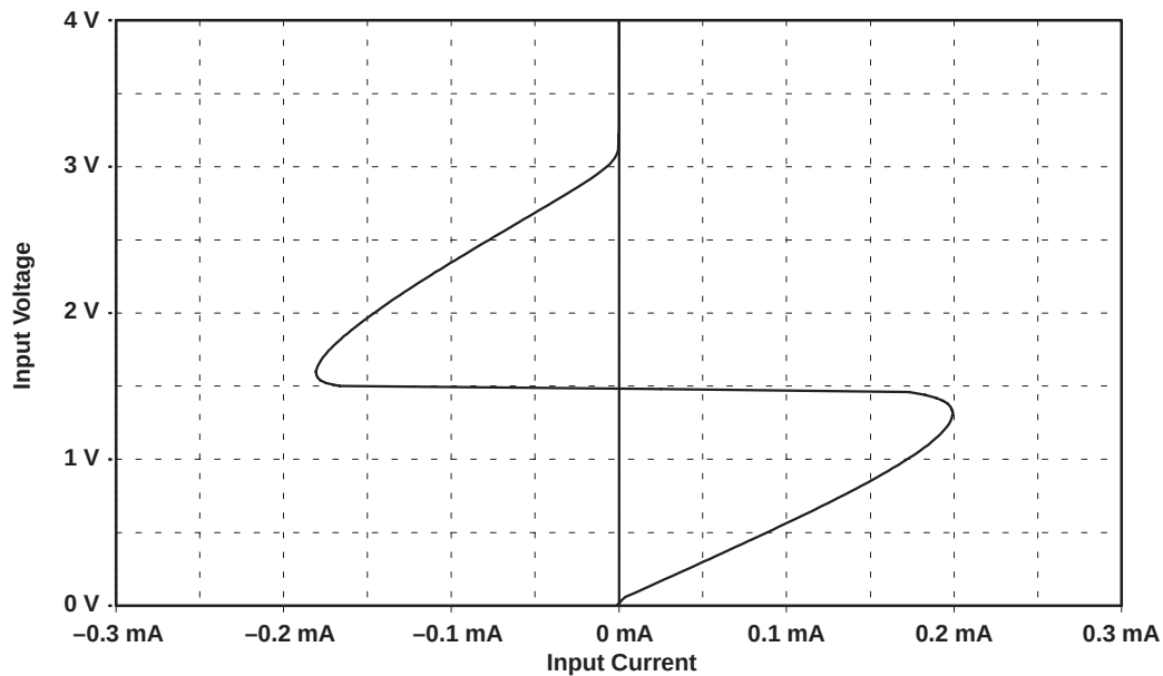
Figure 17. Bus-Hold Characteristics at LVTTL Input of SN74GTLP1655
