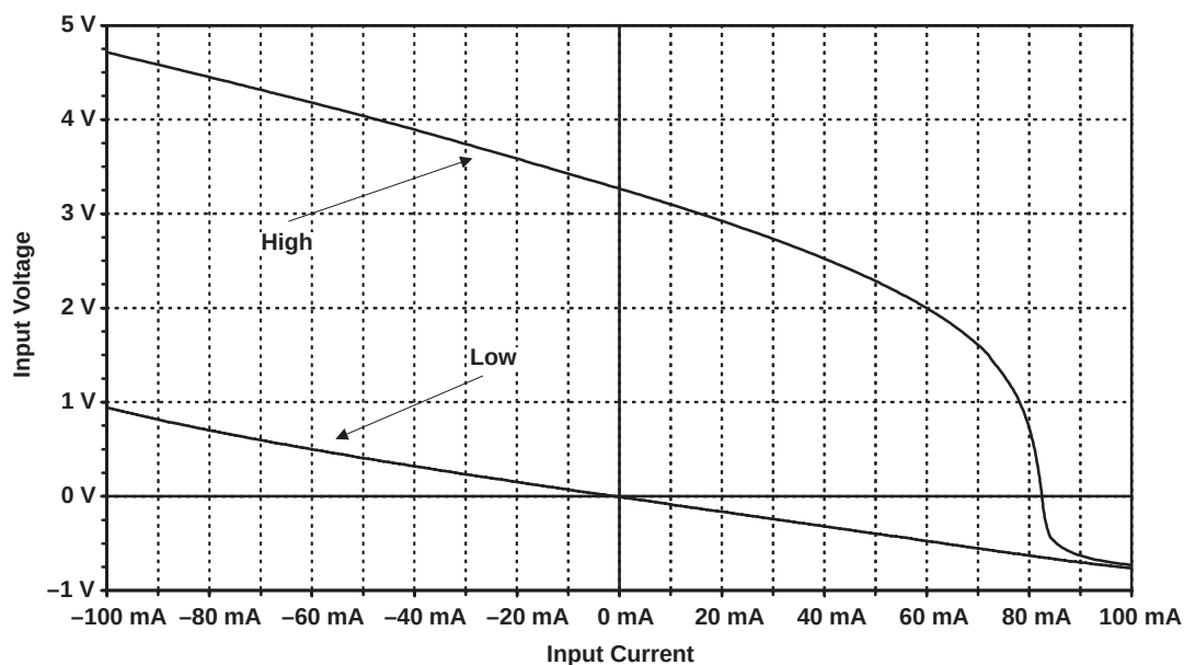
Figure 20. Output Characteristics of LVTTL Side of SN74GTLPH1655
