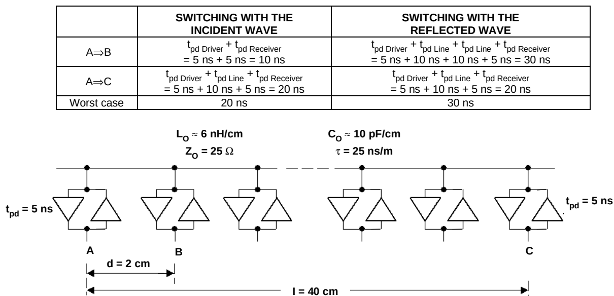
Figure 6. Reflected-Wave Switching
