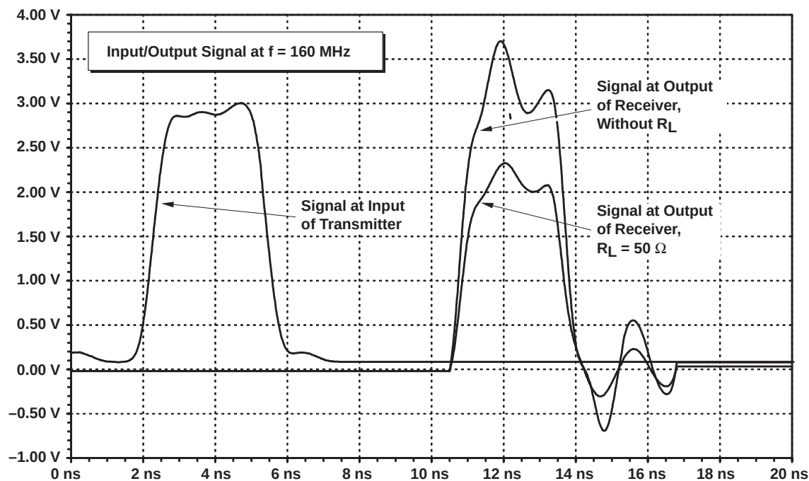
Figure 39. LVTTL Input and Output Signal of SN74GTLPH1655, ERC = GND, Unloaded, 160 MHz
