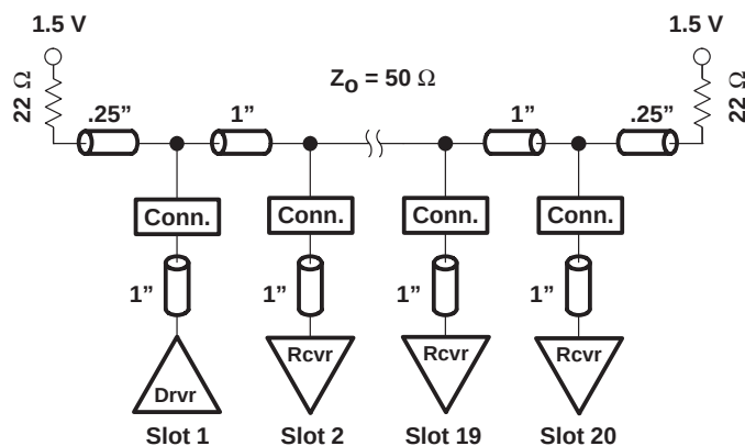
Figure 3. Typical Backplane Physical Representation
