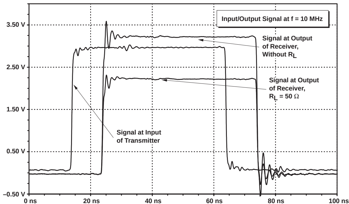
Figure 31. LVTTL Input and Output Signal of SN74GTLPH1655, ERC = GND, Unloaded, 10 MHz
