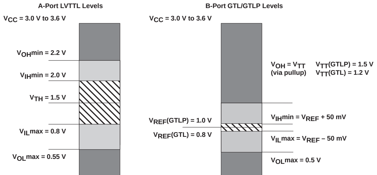
Figure 13. LVTTL and GTLP Signal Levels of SN74GTLPH1655
