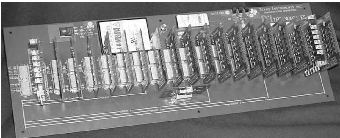
Figure 15. GTLP Demonstration Backplane
