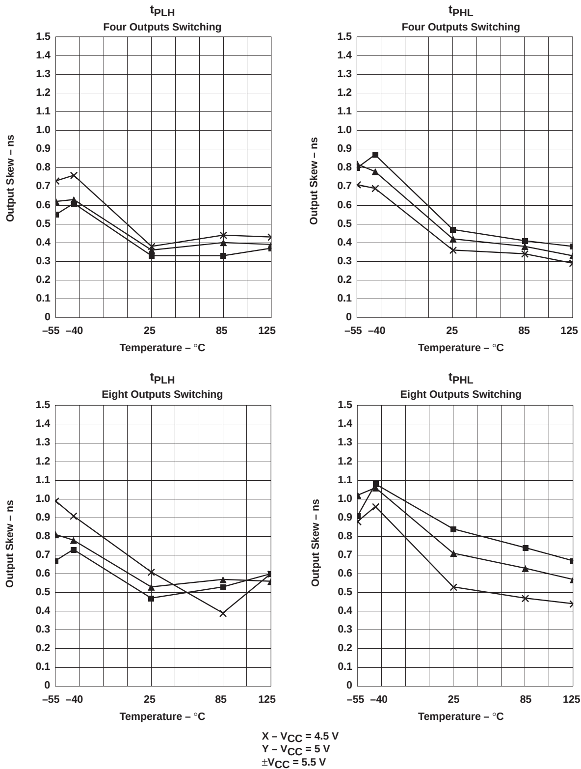
Figure 9. 'ABT244 - Multiple-Output Switching
