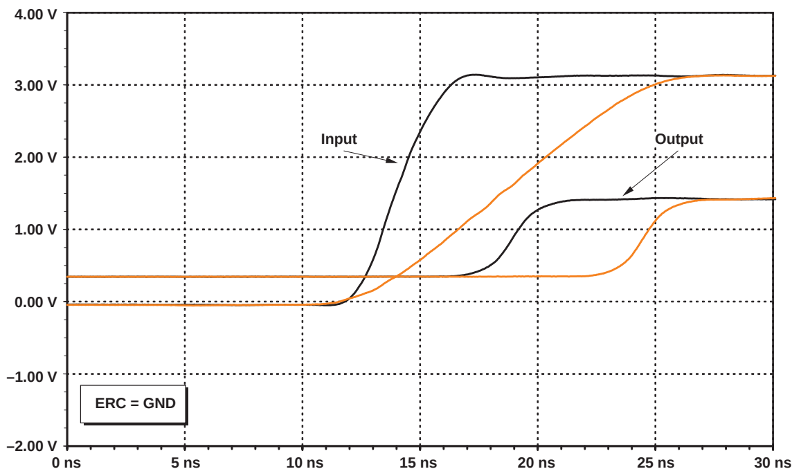
Figure 26. Rising Edge, ERC = GND (Fast Edges), Input Signals t_r = 2 ns, 10 ns
