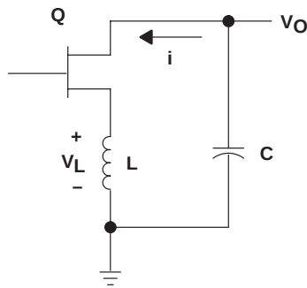
Figure 21. Simultaneous-Switching Output Model
