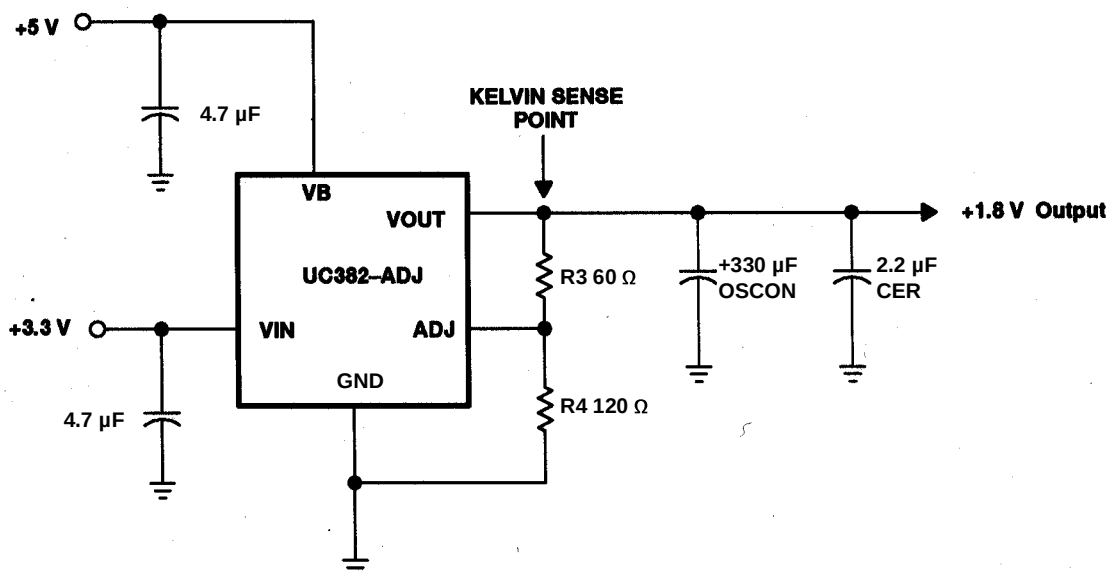
Figure 16. Kelvin-Sensing Circuit
