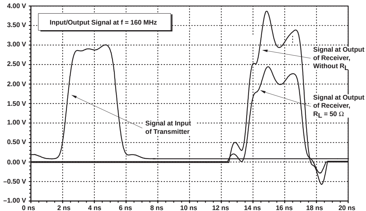
Figure 37. LVTTL Input and Output Signal of SN74GTLPH1655, ERC = V_{CC} , Unloaded, 160 MHz
