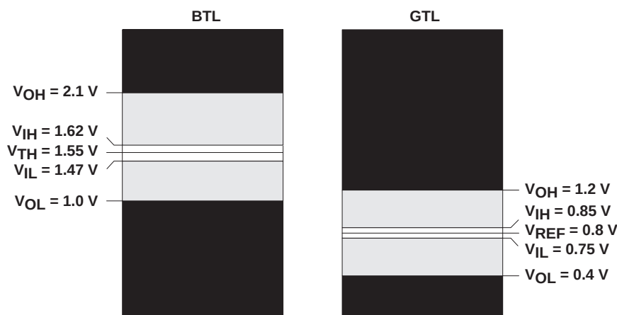
Figure 11. Comparison of Logic Voltage Levels of BTL and GTL
