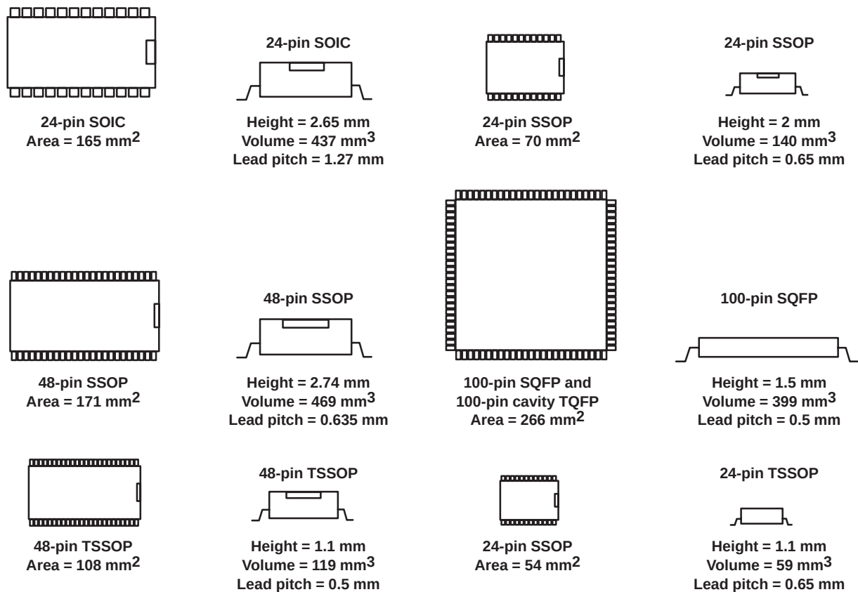
Figure 17. Advanced Packages
