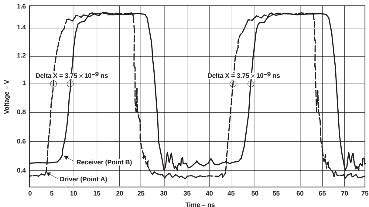
Figure 10. Matched Line Termination
