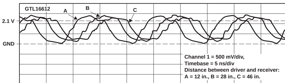
Figure 16. GTL16612 Signal Integrity at the Receiver Input Using Different-Length Cables
