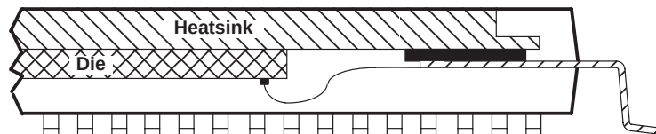
Figure 19. Cross-Section of Thermally Enhanced EIAJ 100-Pin TQFP
