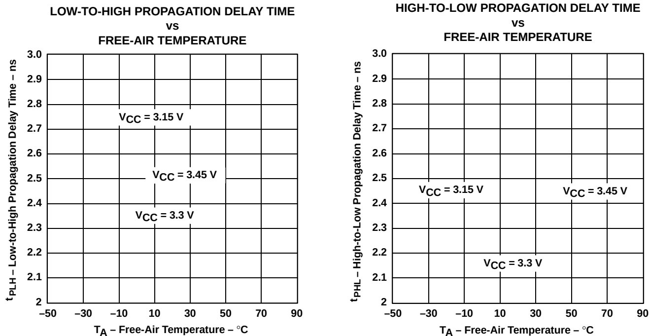
Figure 11. Bus Transceiver Propagation Delay
