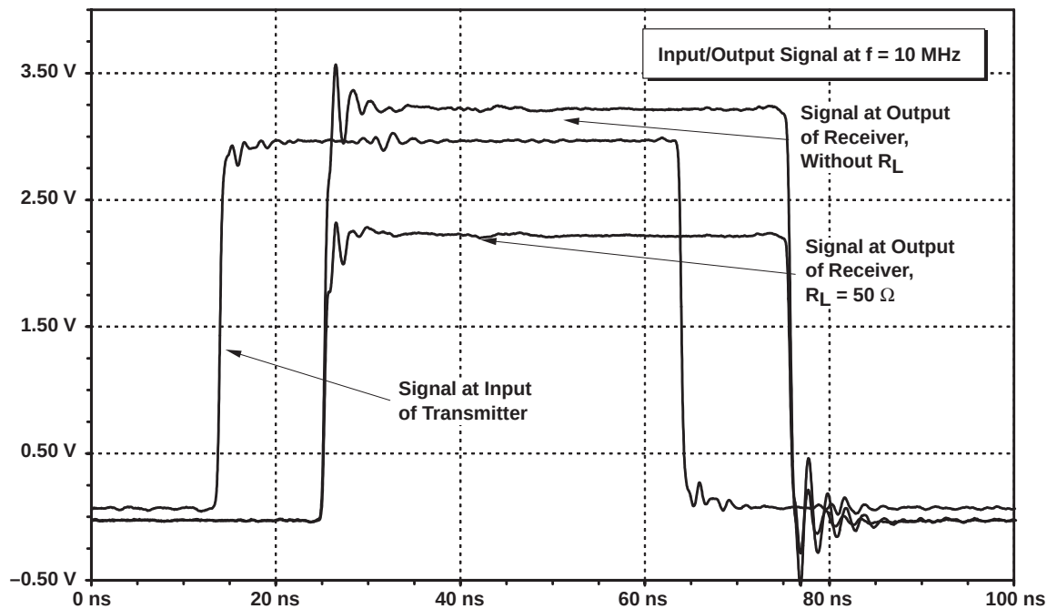
Figure 29. LVTTL Input and Output Signal of SN74GTLP1655, ERC = V_{CC} , Unloaded, 10 MHz
