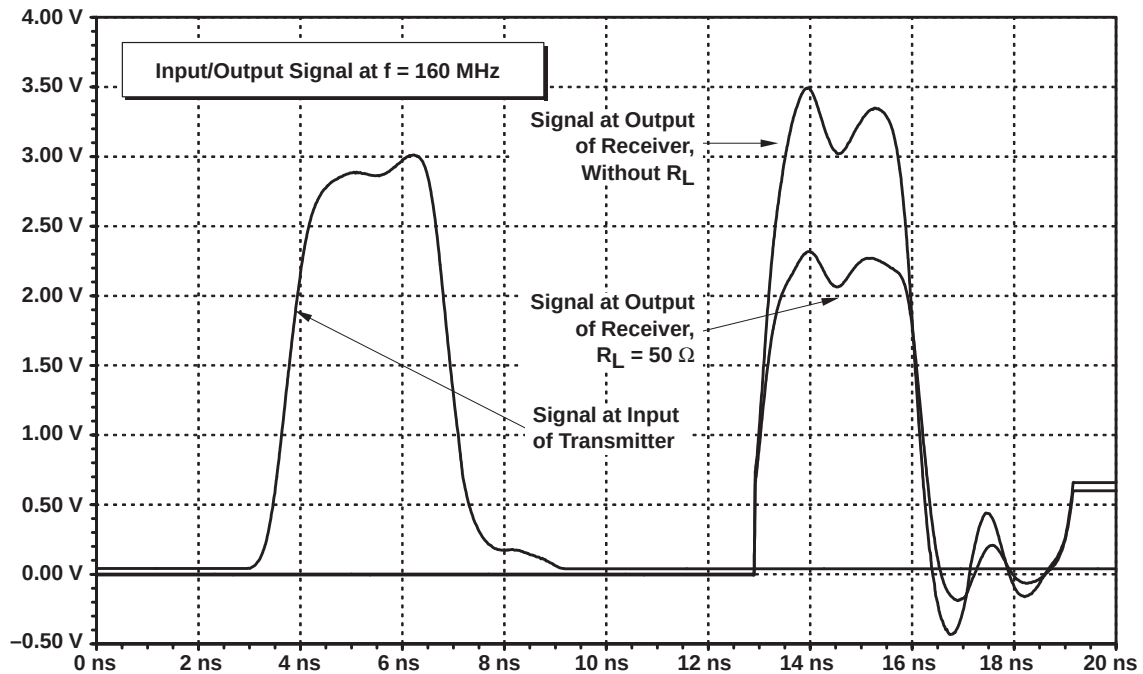
Figure 51. LVTTL Input and Output Signal of SN74GTLPH1655, ERC = GND, Loaded, 160 MHz
