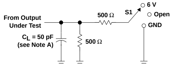
LOAD CIRCUIT FOR Y OUTPUTS
