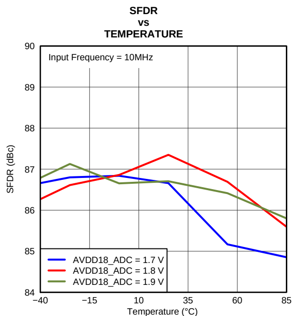
Figure 7-11. SFDR Across Temperature and ADC Analog Supply
