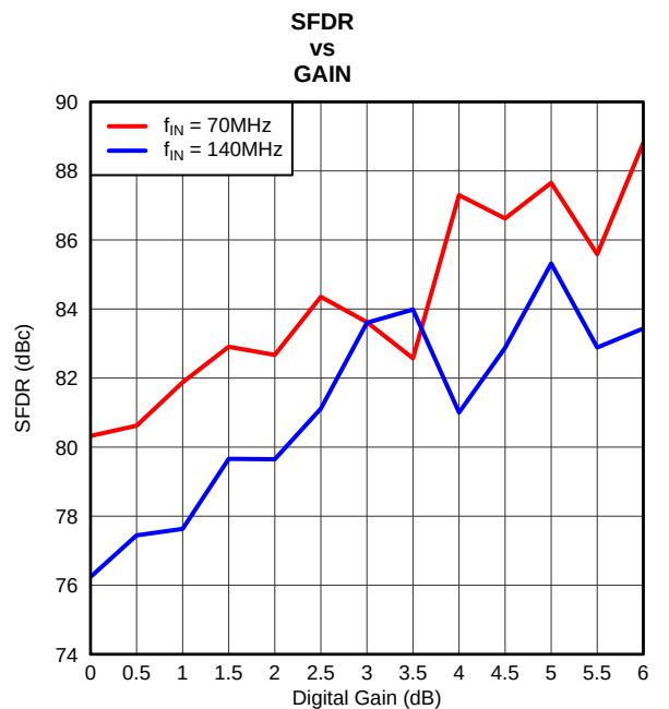
Figure 7-9. SFDR vs Gain
