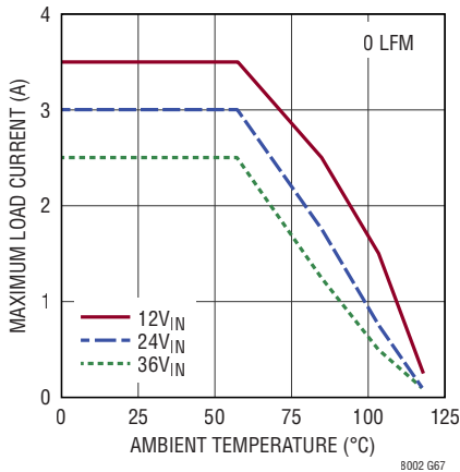
Derating, I-Grade, V_{OUT} = 5V , BIAS = 5V, DC2501A Demo Board
