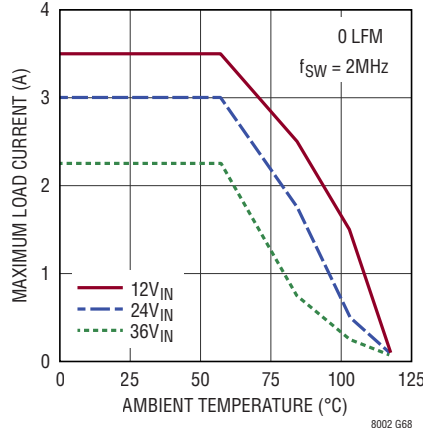
Derating, I-Grade, V_{OUT} = 5V , BIAS = 5V, DC2501A Demo Board
