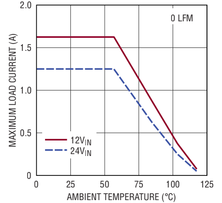
Derating, I-Grade, V_{OUT} = -8\text{V} , BIAS Tied to LTM8002 GND, DC2501A Demo Board
