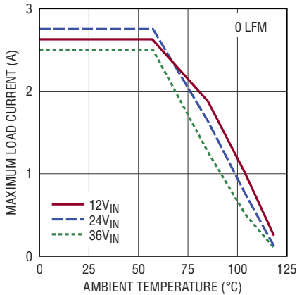
Derating, I-Grade, V_{OUT} = -3.3\text{V} , BIAS Tied to LTM8002 GND, DC2501A Demo Board
