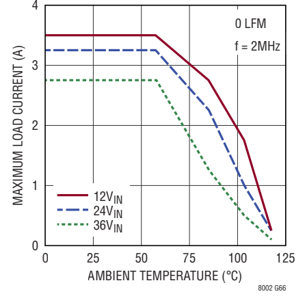
Derating, I-Grade, V_{OUT} = 3.3V , BIAS = 5V, DC2501A Demo Board
