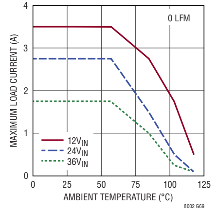
Derating, I-Grade, V_{OUT} = 8V , BIAS = 5V, DC2501A Demo Board
