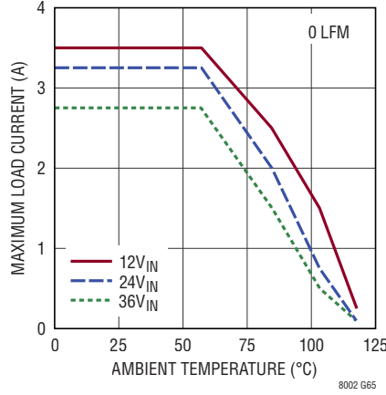
Derating, I-Grade, V_{OUT} = 3.3V , BIAS = 5V, DC2501A Demo Board
