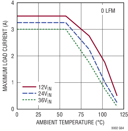
Derating, I-Grade, V_{OUT} = 2.5V , BIAS = 5V, DC2501A Demo Board
