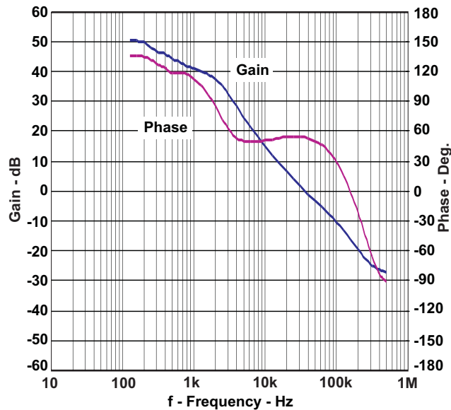
Figure 6. TPS54232EVM-415 Loop Response
