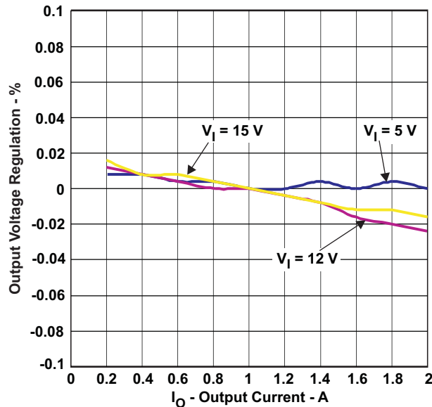
Figure 3. TPS54232EVM-415 Load Regulation
