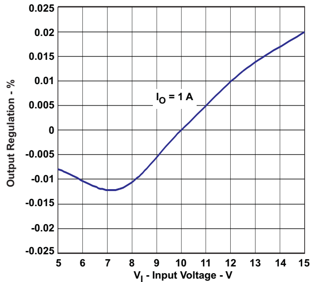
Figure 4. TPS54232EVM-415 Line Regulation
