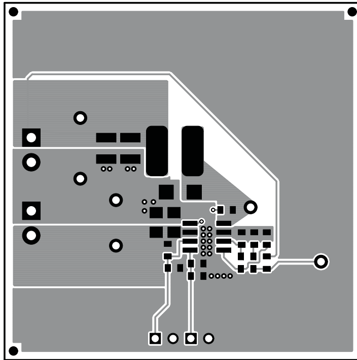
Figure 12. TPS54232EVM-415 Top-Side Layout
