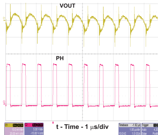
Figure 7. TPS54232EVM-415 Output Ripple
