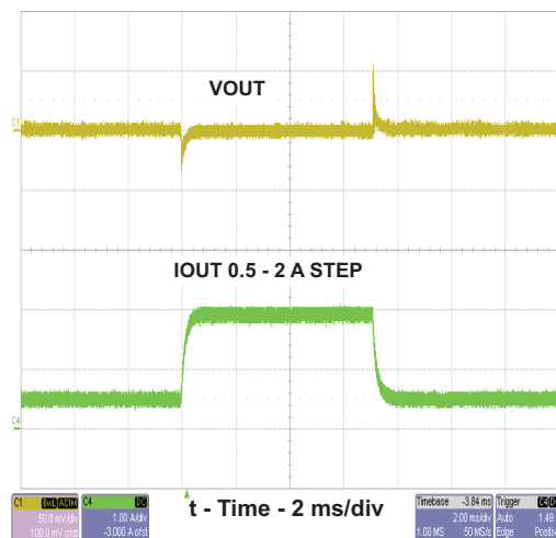
Figure 5. TPS54232EVM-415 Transient Response
