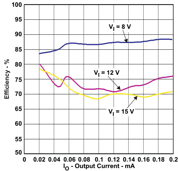
Figure 2. TPS54232EVM-415 Low Current Efficiency
