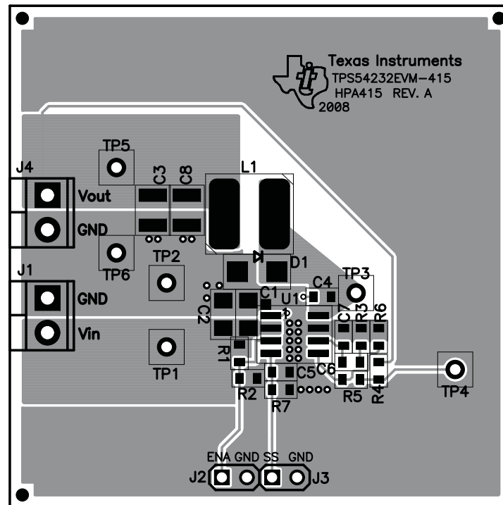
Figure 14. TPS54232EVM-415 Top-Side Assembly
