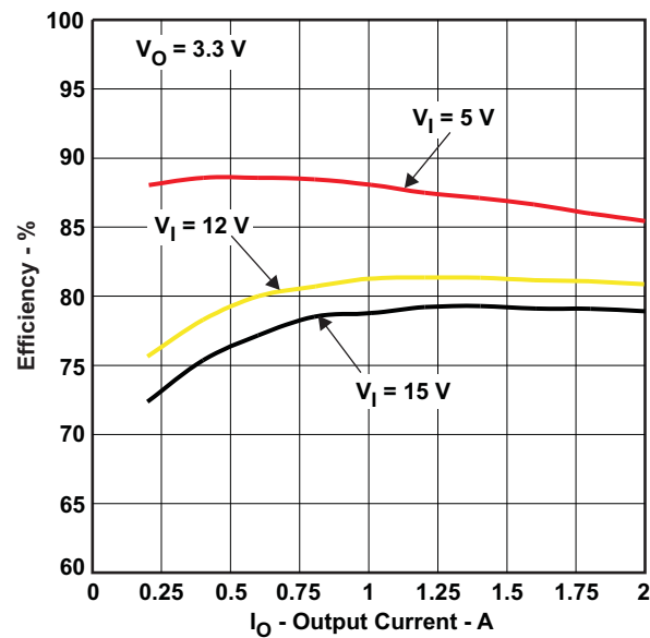
Figure 1. TPS54232EVM-415 Efficiency
