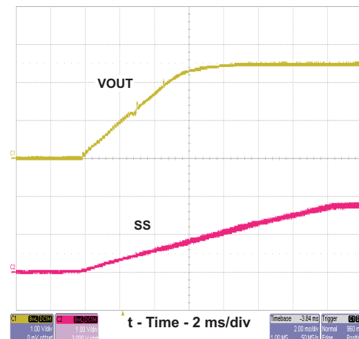
Figure 10. TPS54232EVM-415 Start-up Relative to Enable
