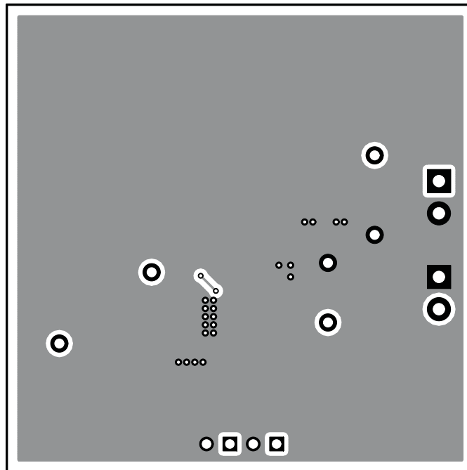
Figure 13. TPS54232EVM-415 Bottom-Side Layout
