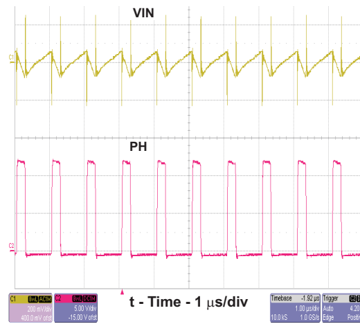
Figure 8. TPS54232EVM-415 Input Ripple
