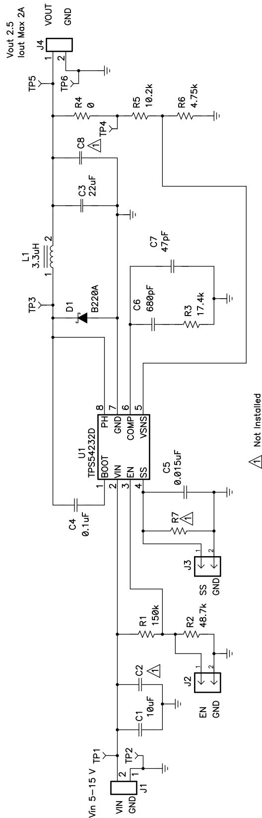
Figure 15. TPS54232EVM-415 Schematic
