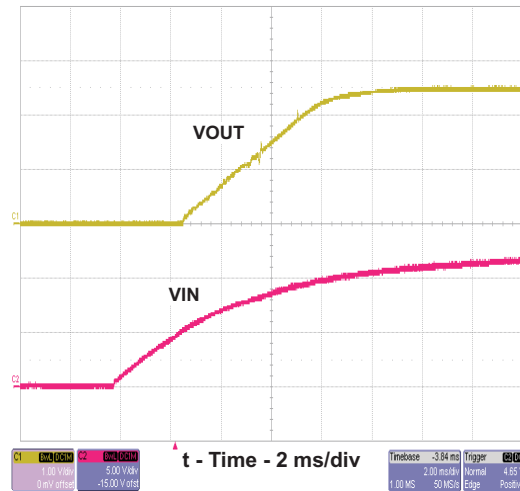
Figure 9. TPS54232EVM-415 Start-Up Relative to V_{IN}
