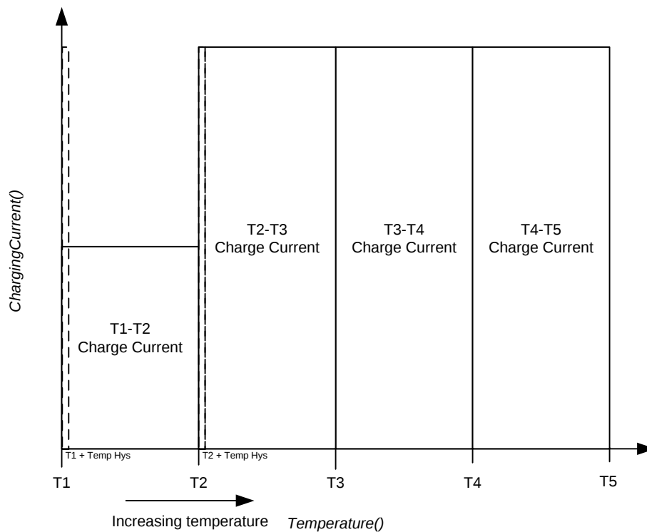
Figure 2-7. Temperature Hysteresis for Charging Current
