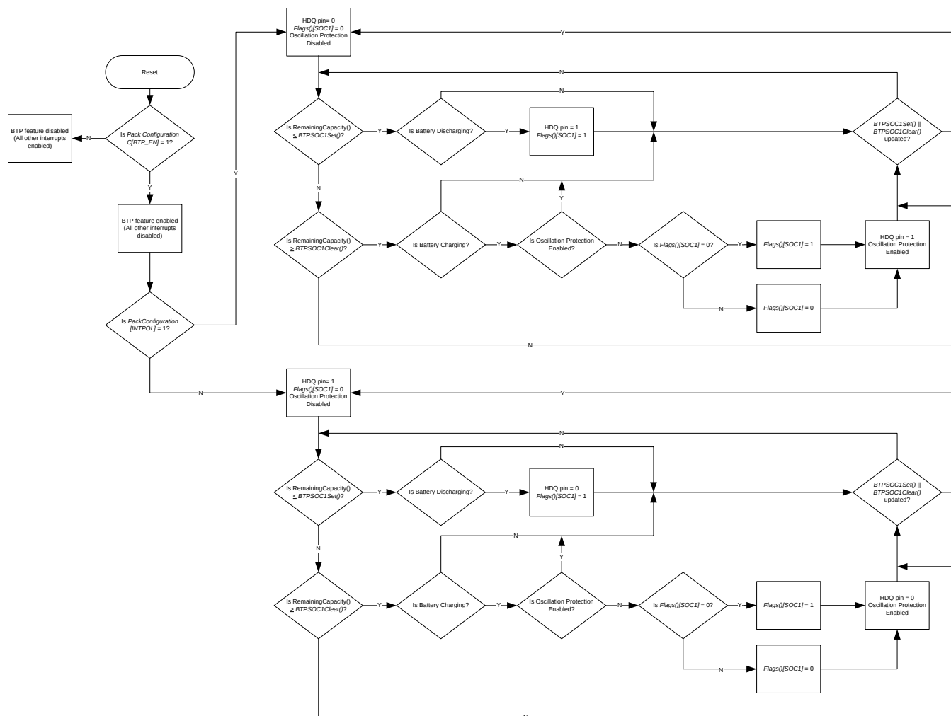
Figure 2-1. BTP Algorithm Flow
