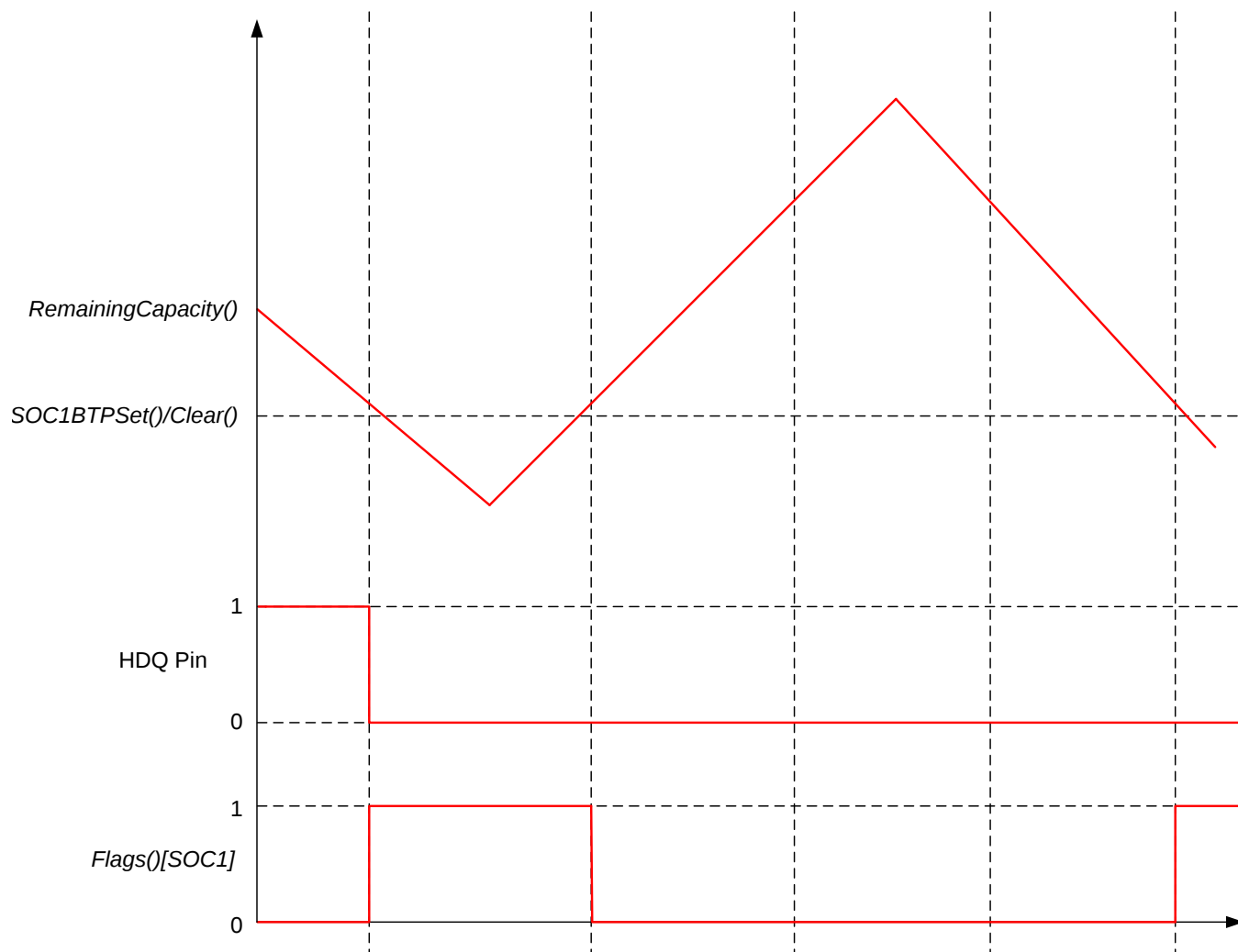
Figure 2-3. BTP Configuration with Shared Thresholds
