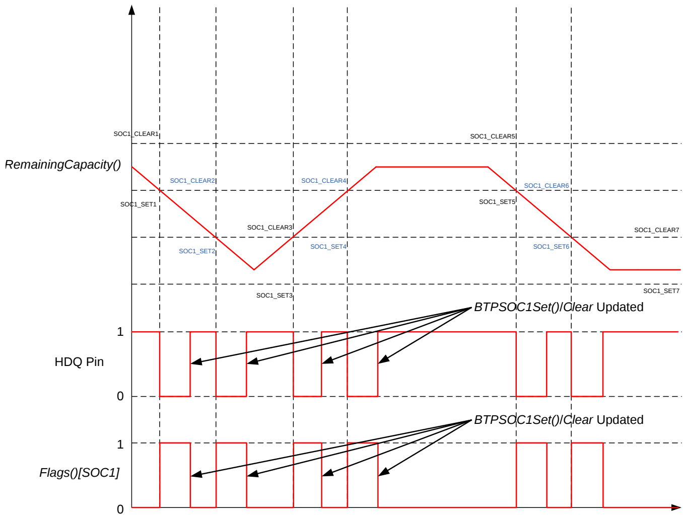
Figure 2-2. BTP Configuration with Multiple Thresholds
