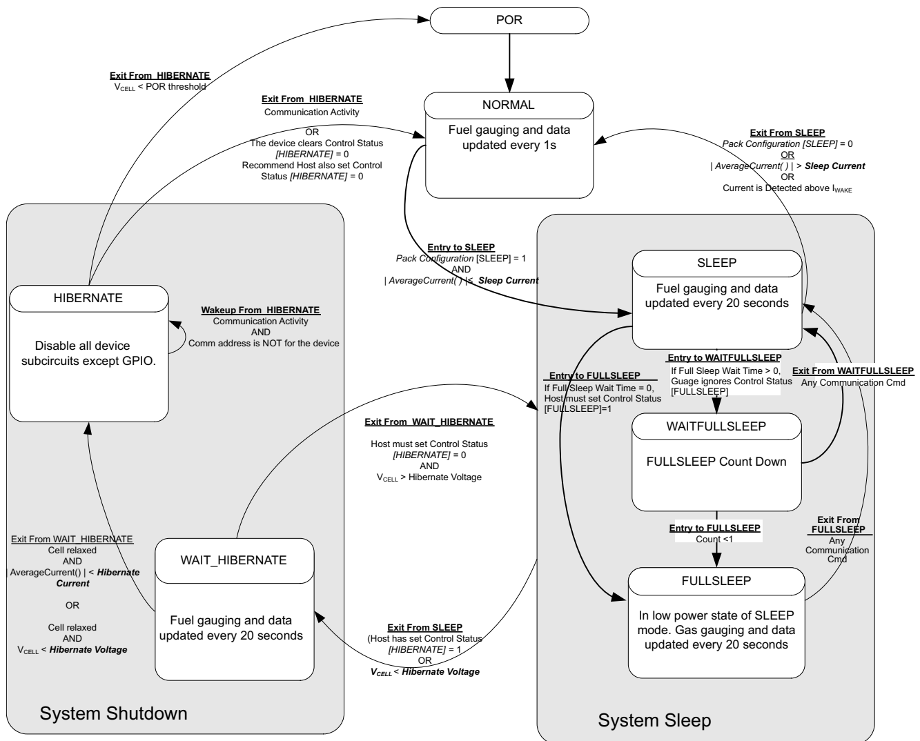
Figure 2-9. Power Mode Diagram—System Sleep
