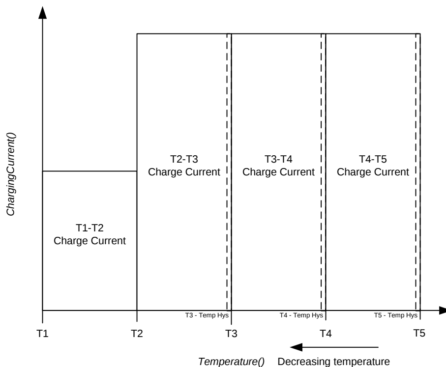
Figure 2-8. Temperature Hysteresis for Charging Voltage
