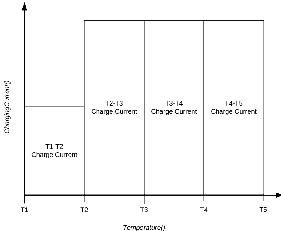
Figure 2-5. JEITA Charging Current Profile
