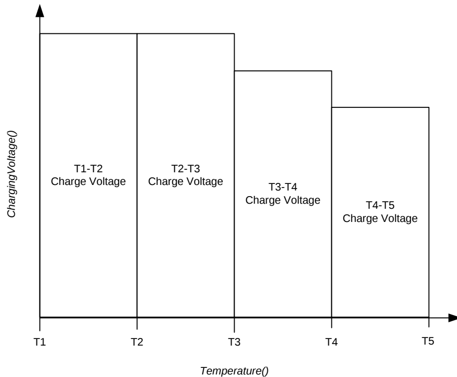
Figure 2-6. JEITA Charging Voltage Profile
