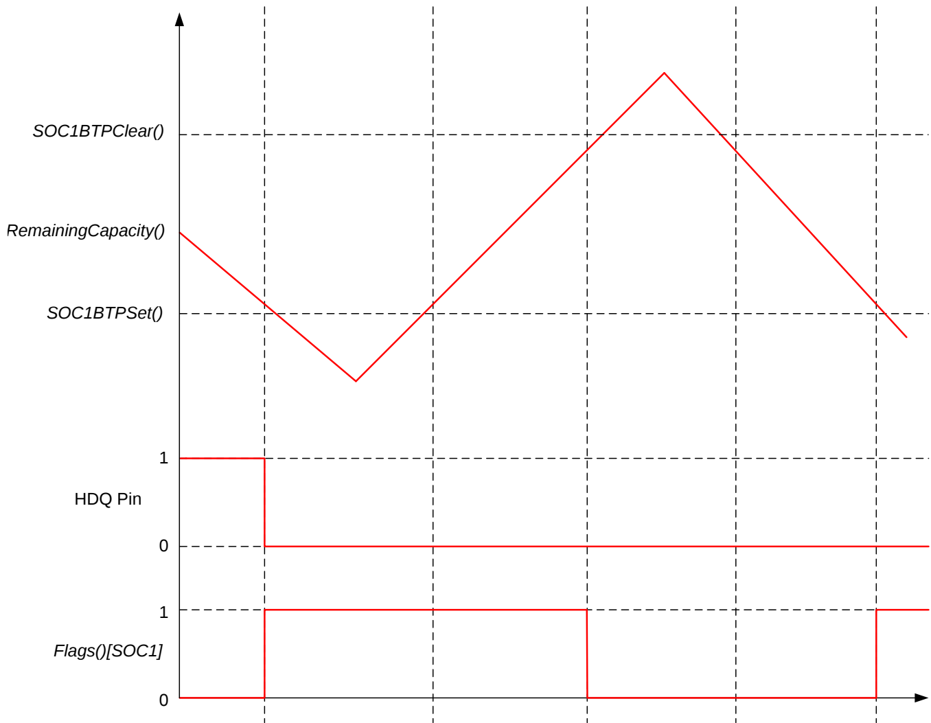
Figure 2-4. BTP Configuration with Separate Thresholds
