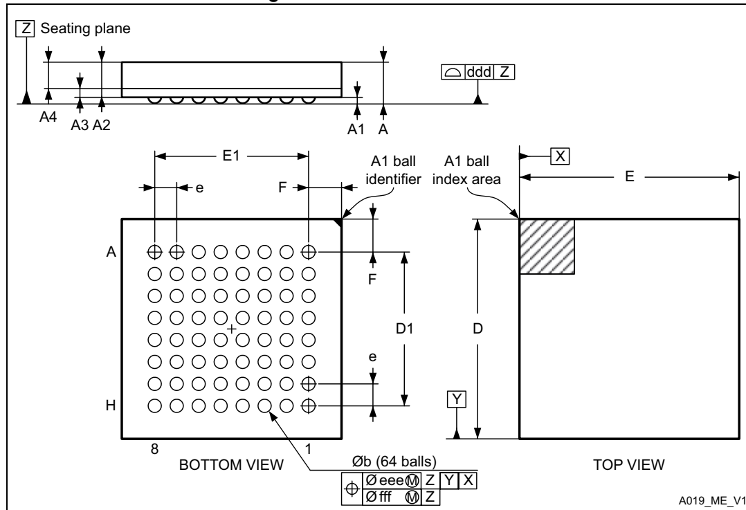
Figure 61. UFBGA64 - outline
