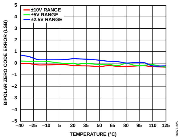
Figure 25. Bipolar Zero Code Error vs. Temperature
