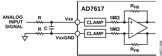
Figure 44. Input Resistance Matching on the Analog Input
