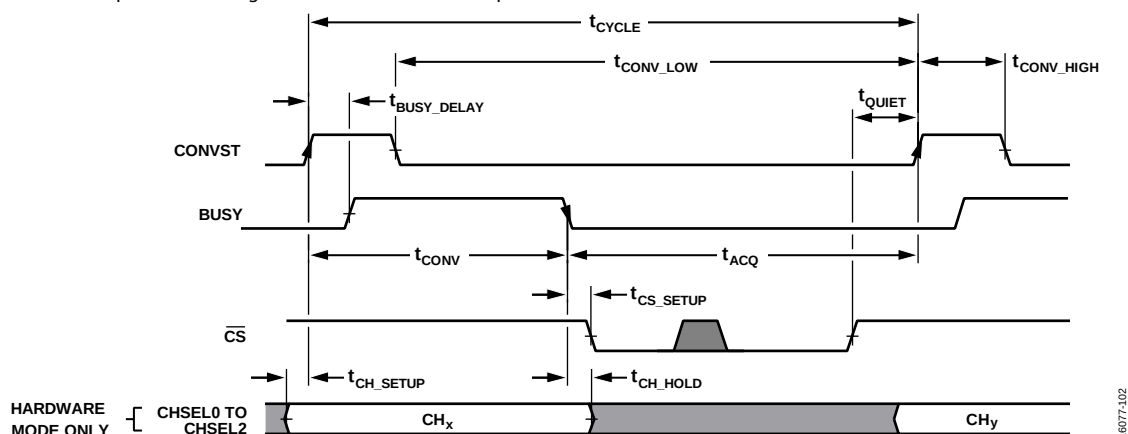
Figure 2. Universal Timing Diagram Across All Interfaces
