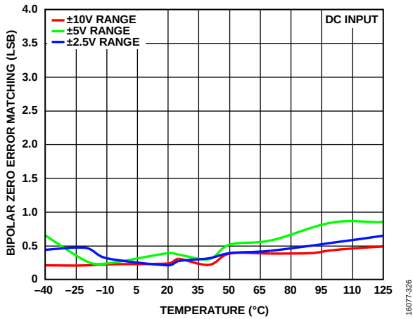
Figure 26. Bipolar Zero Code Error Matching vs. Temperature
