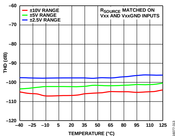
Figure 13. THD vs. Temperature
