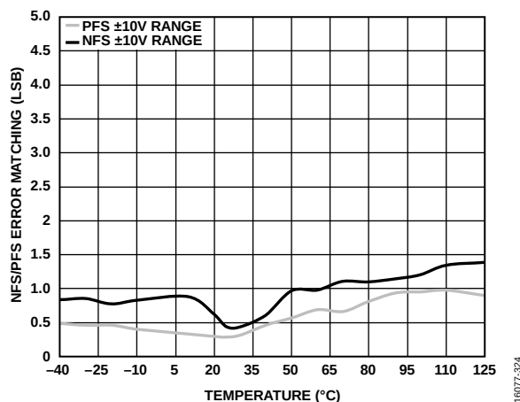
Figure 24. NFS/PFS Error Matching vs. Temperature
