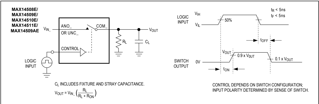
Figure 2. Switching Time
