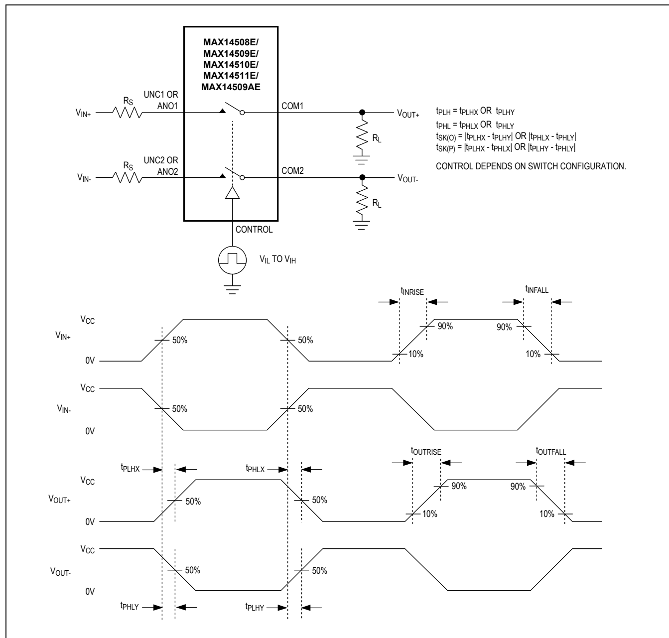
Figure 3. Output Skew
