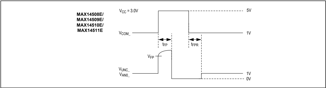
Figure 1. Fault Protection
