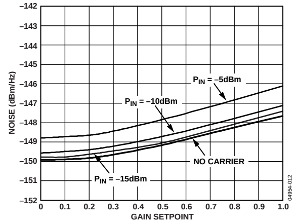
Figure 12. Output Noise Floor vs. Gain Setpoint, No Carrier, with Carrier (20 MHz Offset), RF P IN = -5, -10, -15, No Carrier, RF Frequency = 380 MHz
