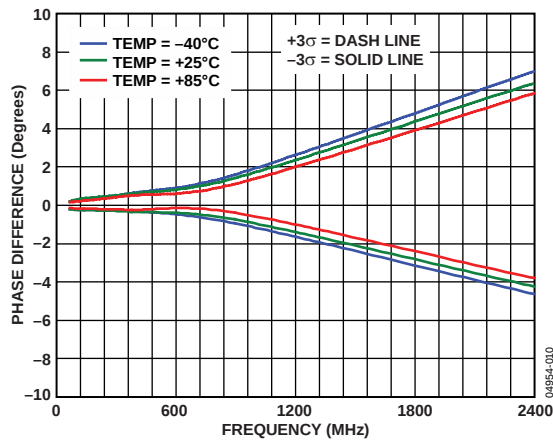
Figure 10. Channel-to-Channel Phase Matching vs. RF Frequency, Temp = +85°C, +25°C, -40°C, Gain Setpoint = 1.0
