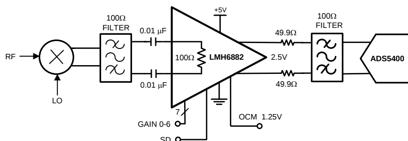
Figure 50. LMH6882 Typical Application
