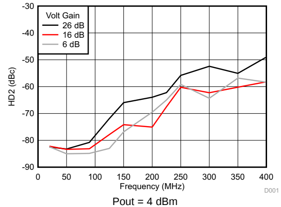
Figure 34. HD2 vs Frequency Across Gain Settings
