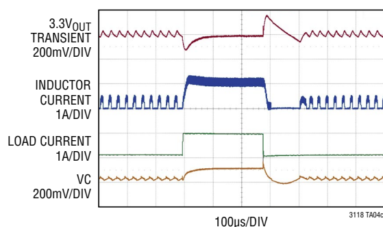
100mA to 1A Load Step, V_{IN} = 12V , V_{OUT} = 3.3V , Auto Burst Mode
