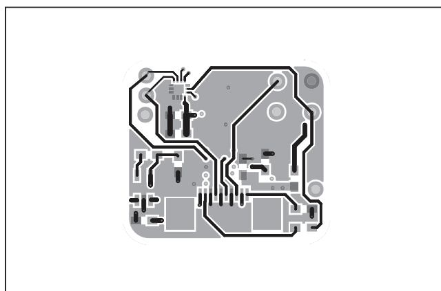
Figure 8. MAX30102 Daughter Board PCB Layout—Layer 2
