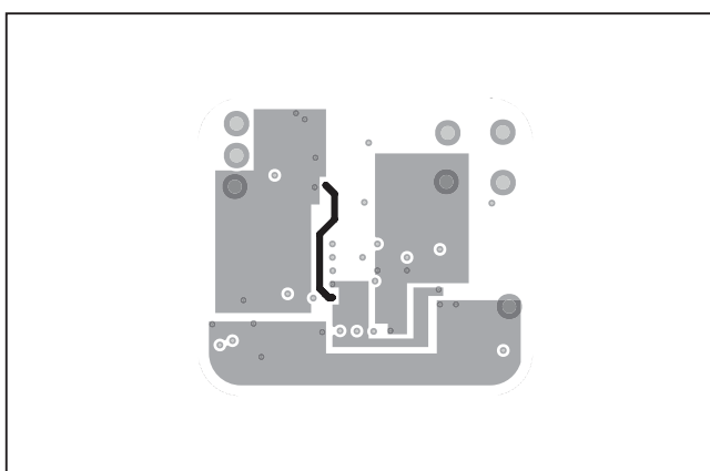
Figure 10. MAX30102 Daughter Board PCB Layout—Component Side
