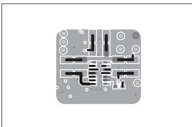
Figure 12. MAX30102 Daughter Board Component Placement Guide—Solder Side
