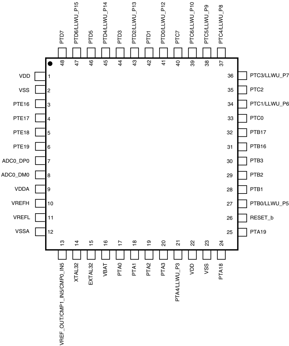
Figure 10-2. K12 48 LQFP Pinout Diagram
