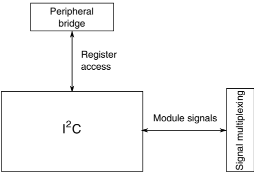
Figure 3-42. I2C configuration
