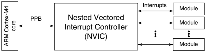
Figure 3-2. NVIC configuration
