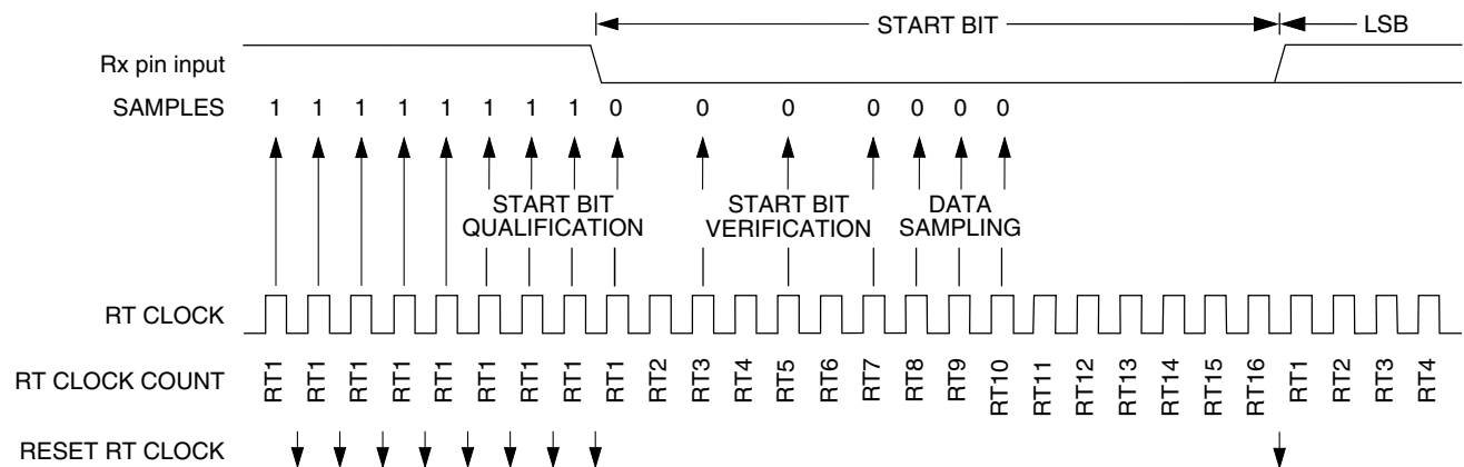
Figure 42-159. Receiver data sampling
