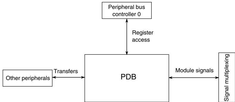
Figure 3-33. PDB configuration
