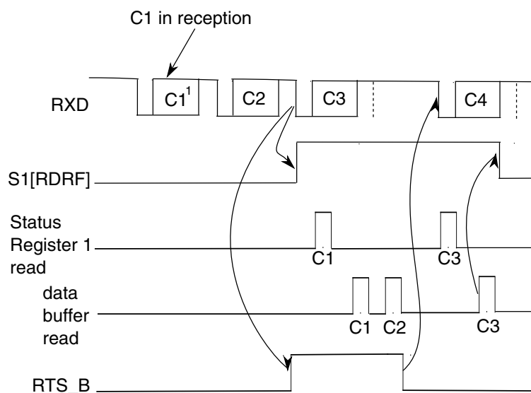
Figure 42-166. Receiver hardware flow control timing diagram
