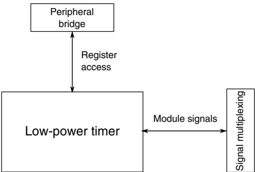
Figure 3-37. LPTMR configuration
