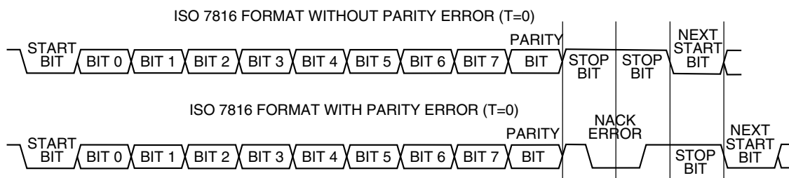
Figure 42-181. ISO-7816 T = 0 data format
