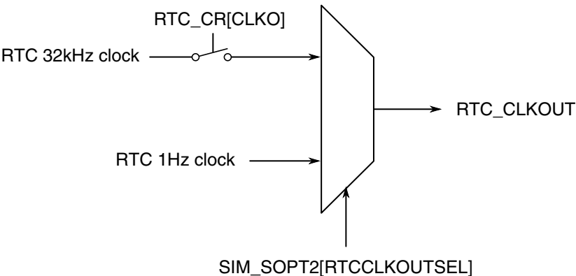
Figure 3-40. RTC_CLKOUT generation
