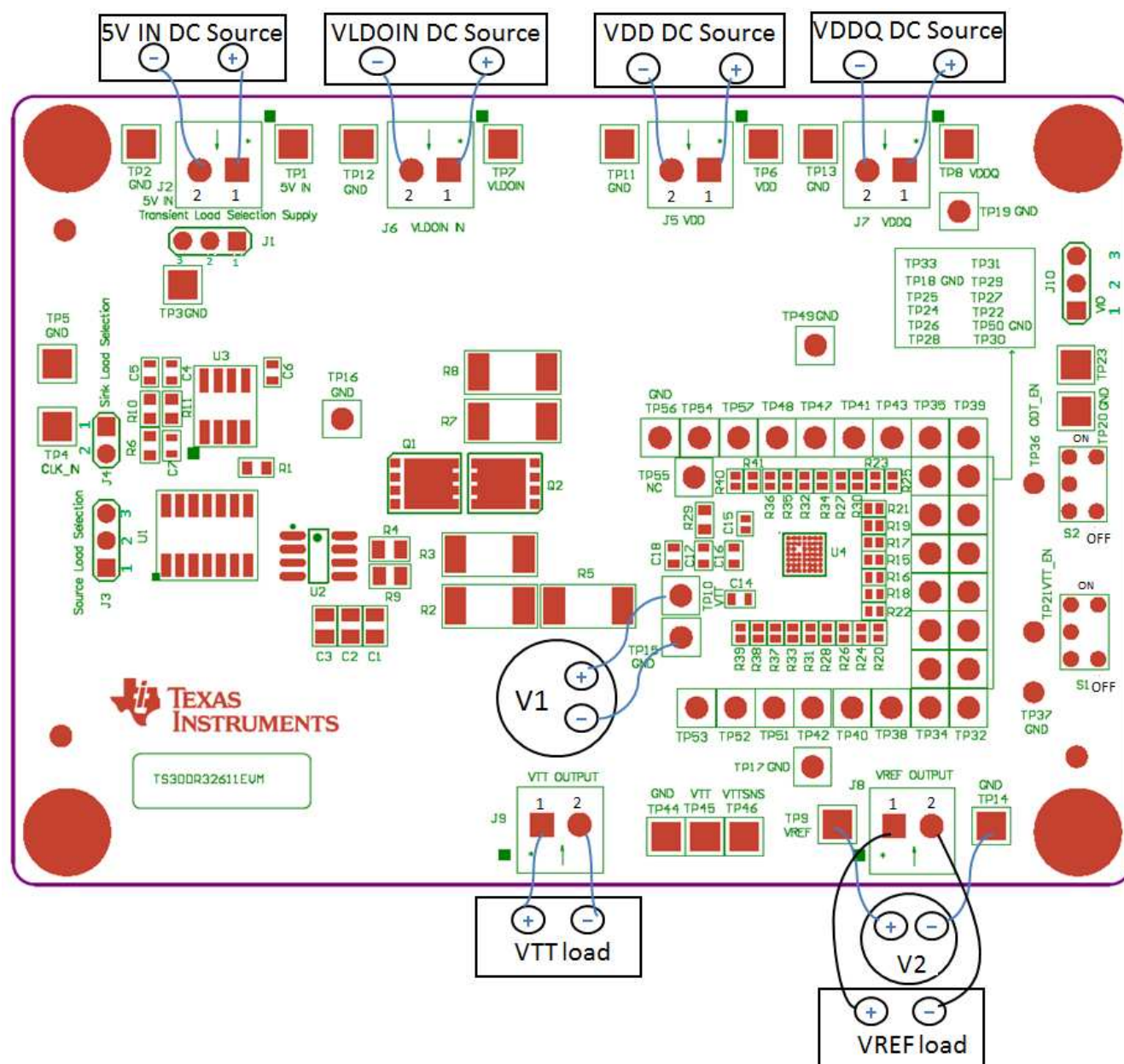
Figure 2. TS3DDR32611 EVM Recommended Test Setup
