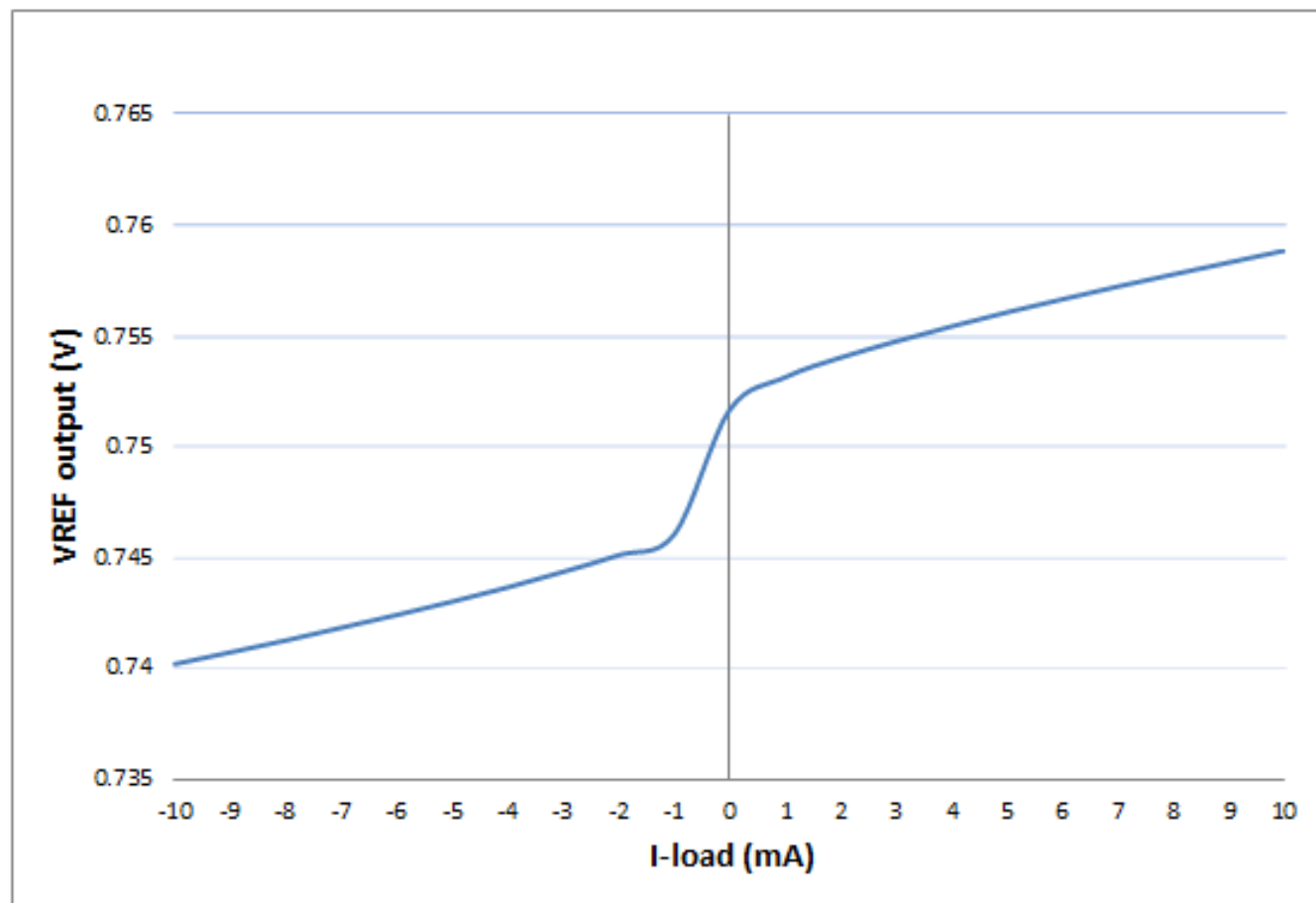
Figure 6. 0.75VREF Load Regulation
