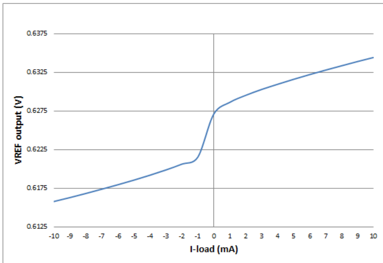
Figure 8. 0.625VREF Load Regulation
