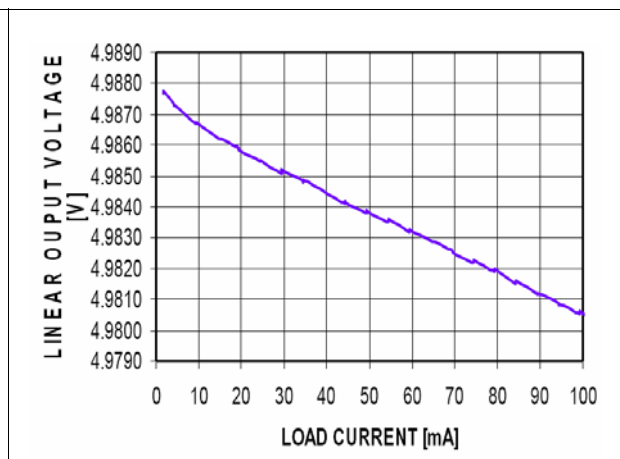
Figure 10. LDO5 vs output current
