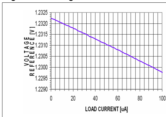
Figure 15. Voltage reference vs load current
