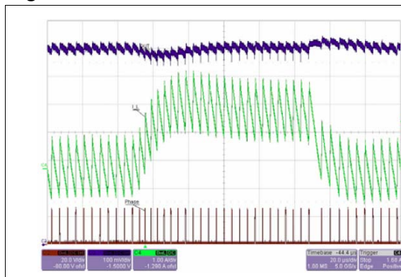
Figure 17. OUT1 = 3.3V load transient 0→2A
