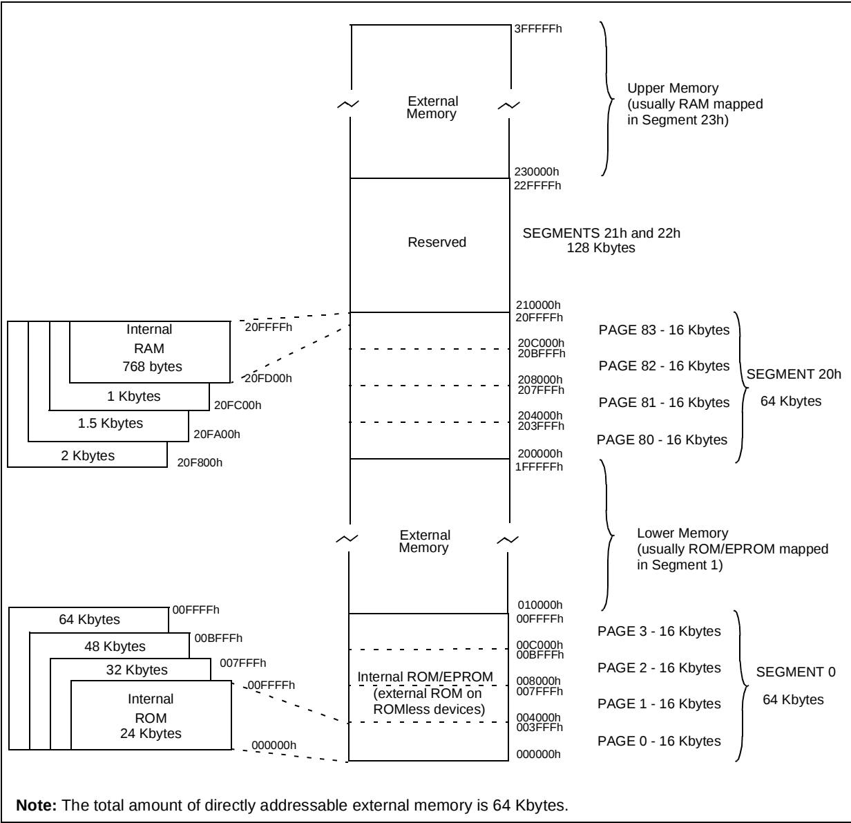
Figure 18. Memory Map
