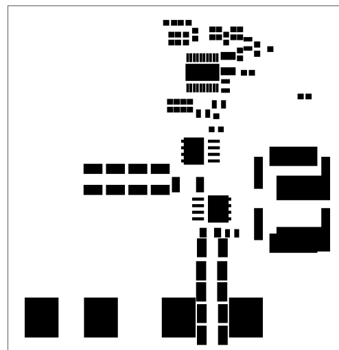
TOP SOLDER PASTE MASK (.LRC) AS VIEWED FROM TOP 881013161-001
