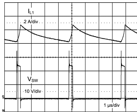
Figure 6. Short Circuit at 24V_{IN} 125°C
