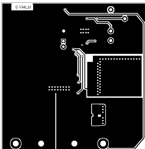
BOTTOM (.SOL) LAYER AS VIEWED FROM TOP 880013161-001
