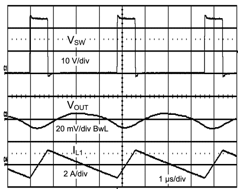
Figure 10. Full Synchronous Operation at 24V IN with JMP1 Removed
