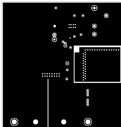
LAYER 2 (.LY2) AS VIEWED FROM TOP 880013161-001
