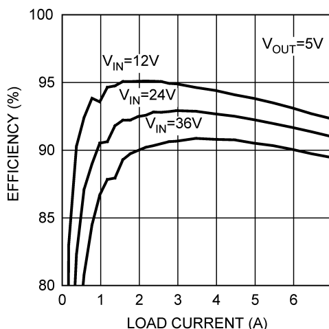
Figure 1. Efficiency with 6 µH Cooper Inductor
