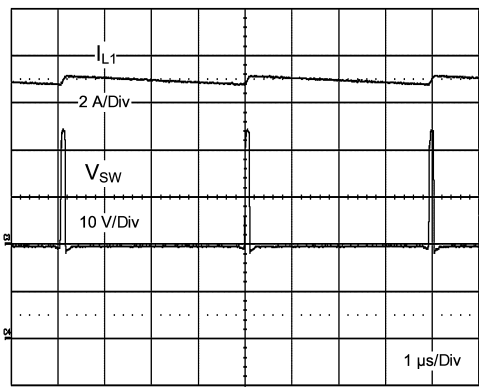
Figure 5. Short Circuit at 24V_{IN} Room Temperature
