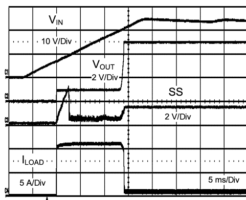
Figure 9. Start-up into Active Load at 24V IN
