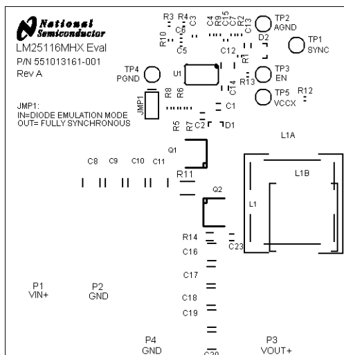
TOP SILKSCREEN (.PLC) AS VIEWED FROM TOP 880013161-001
