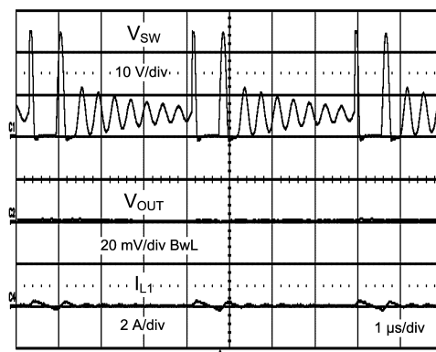
Figure 11. Discontinuous Operation using Diode Emulation Mode at 24V IN with JMP1 Installed
