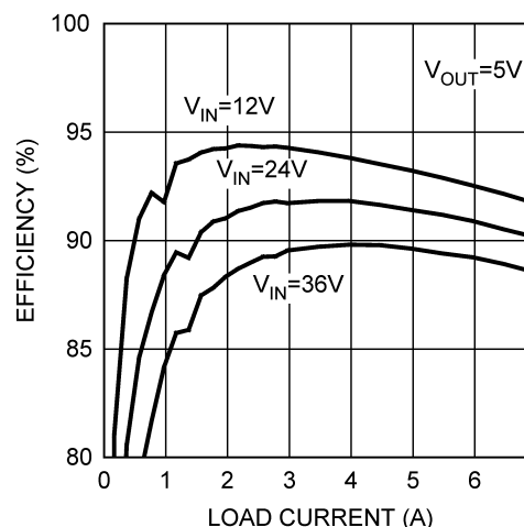
Figure 2. Efficiency with 5.6 µH Pulse Inductor
