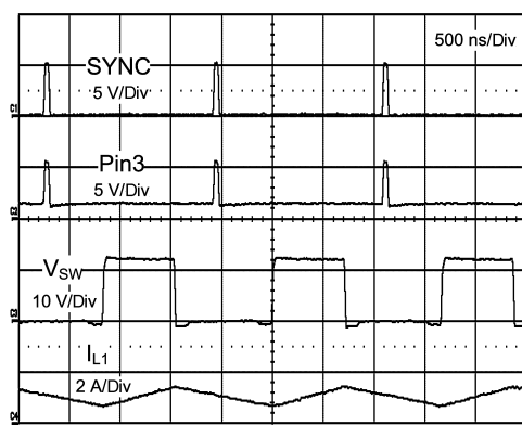
Figure 8. Synchronization at 12V IN
