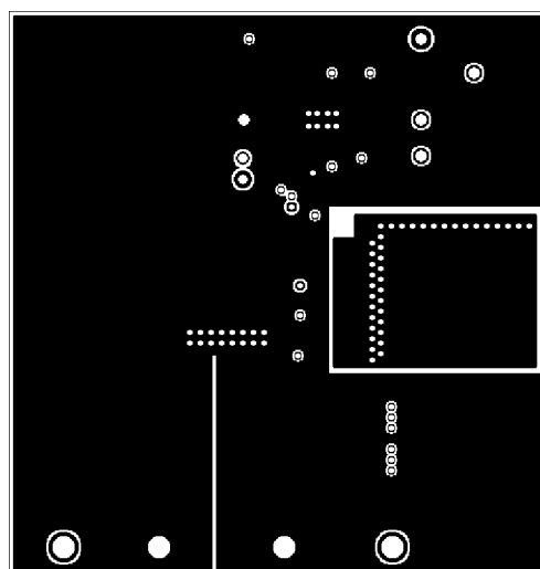
LAYER 3 (.LY3) AS VIEWED FROM TOP 880013161-001
