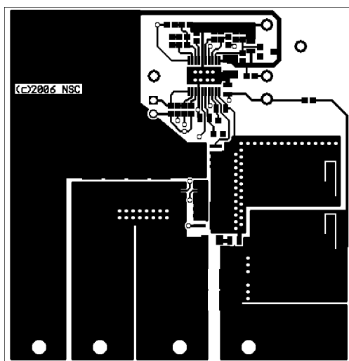
TOP (.CMP) LAYER AS VIEWED FROM TOP 880013161-001
