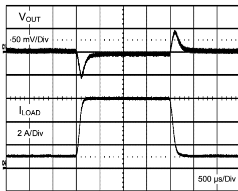
Figure 12. Transient Response at 24V IN
