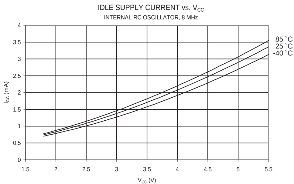
Figure 147. Idle Supply Current vs. V_{CC} (Internal RC Oscillator, 8 MHz)
