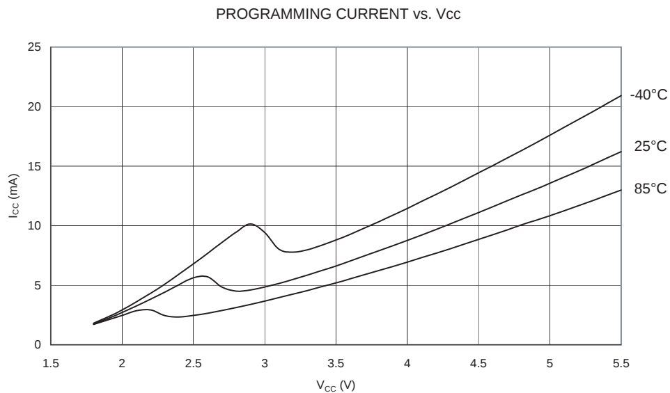
Figure 201. Programming Current vs. V_{CC}
