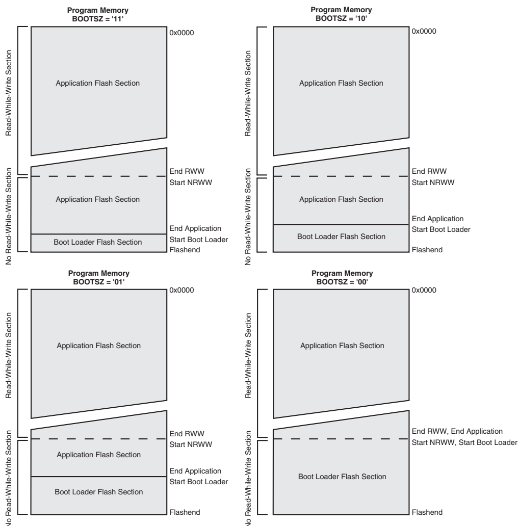
Figure 117. Memory Sections
