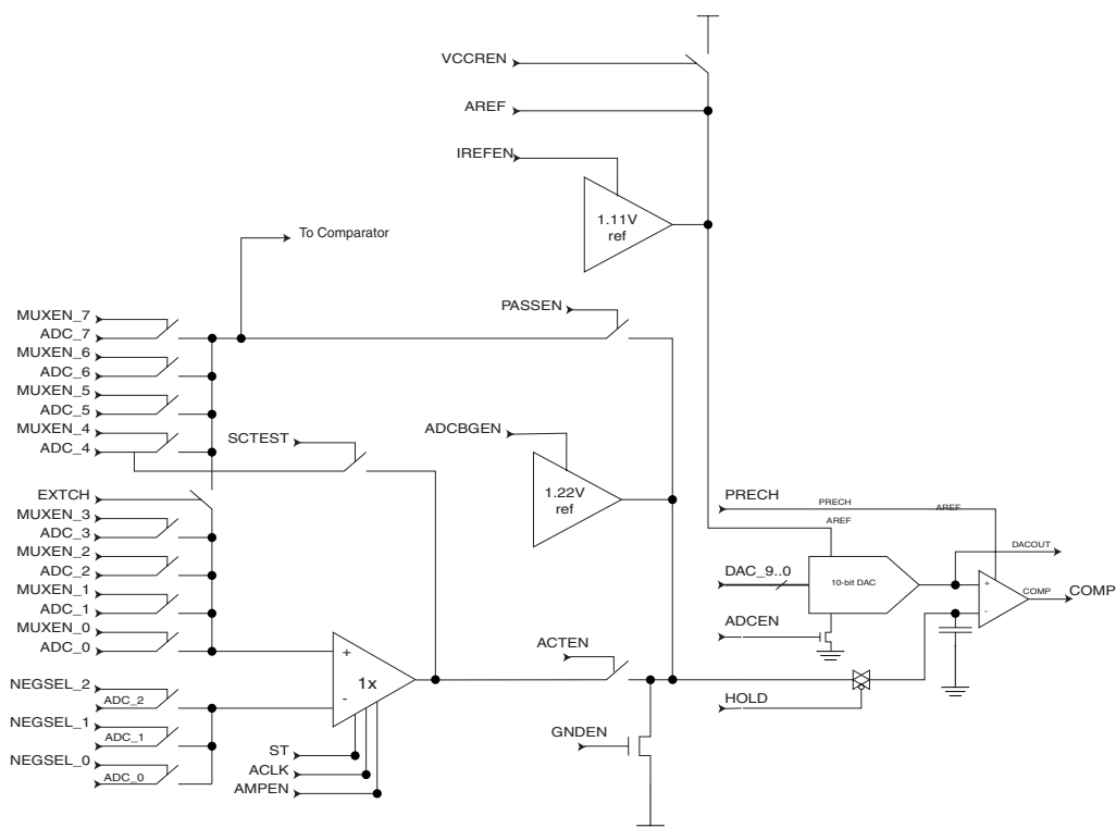
Figure 115. Analog to Digital Converter
