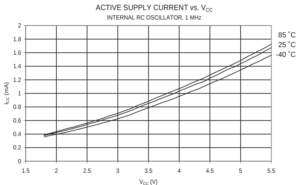
Figure 143. Active Supply Current vs. V_{CC} (Internal RC Oscillator, 1 MHz)
