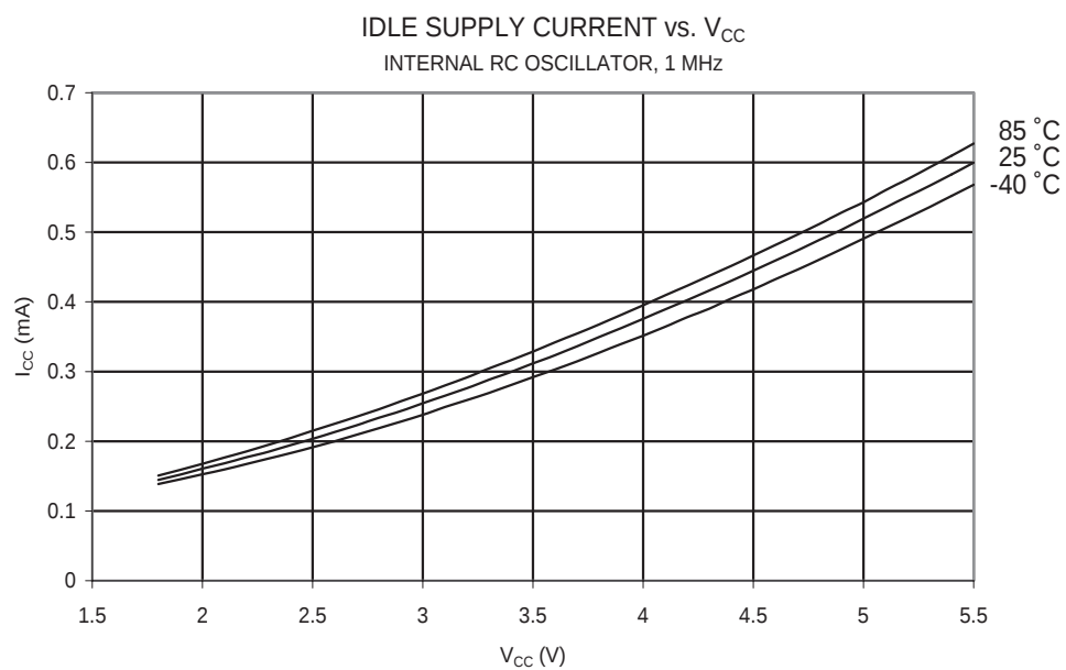
Figure 148. Idle Supply Current vs. V_{CC} (Internal RC Oscillator, 1 MHz)
