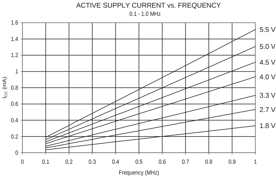
Figure 140. Active Supply Current vs. Frequency (0.1 - 1.0 MHz)
