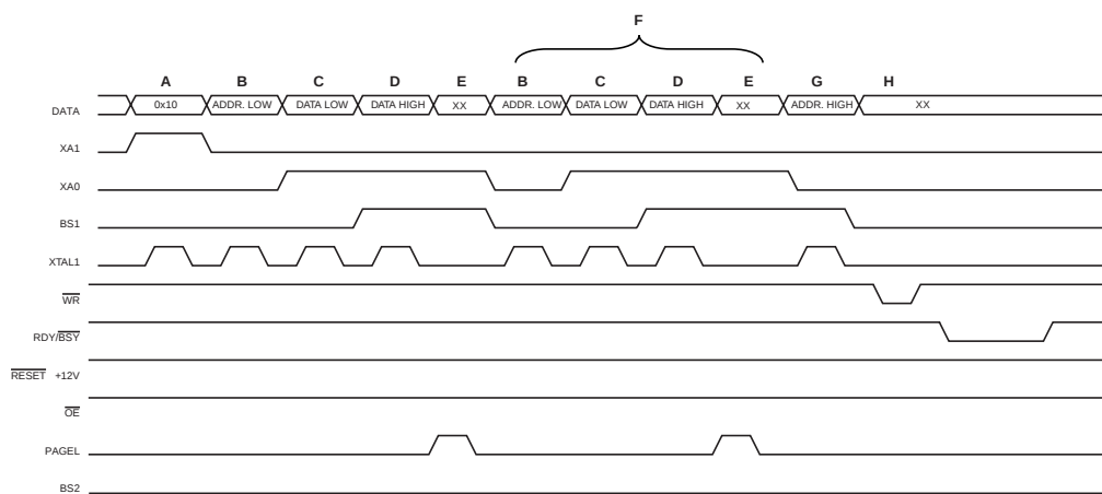
Figure 121. Programming the Flash Waveforms (1)
