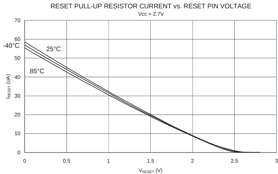
Figure 165. Reset Pull-up Resistor Current vs. Reset Pin Voltage ( V_{CC} = 2.7V )
