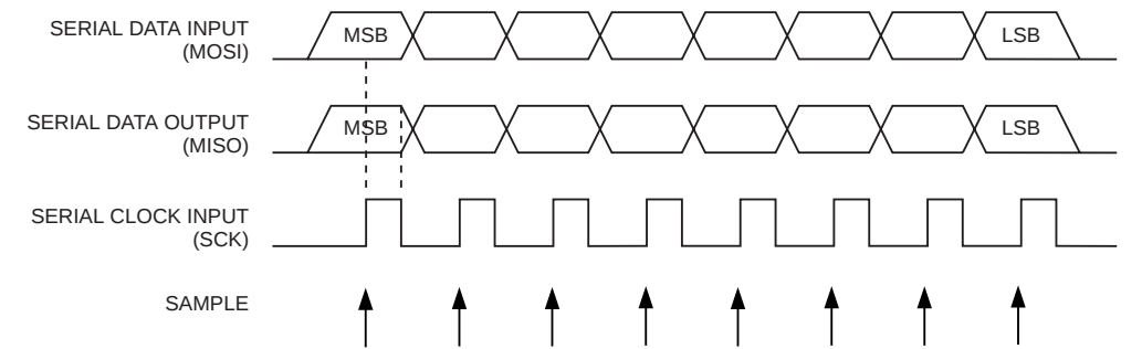
Figure 129. Serial Programming Waveforms
