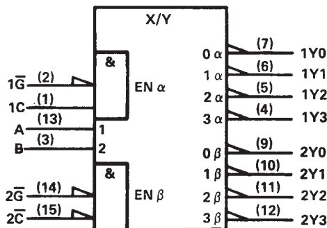
'155, 'LS155A
