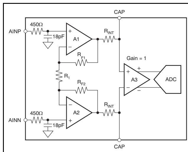
Figure 1. Simplified Diagram of the Amplifier
