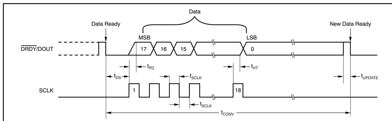
Figure 6. 18-Bit Data Retrieval Timing
