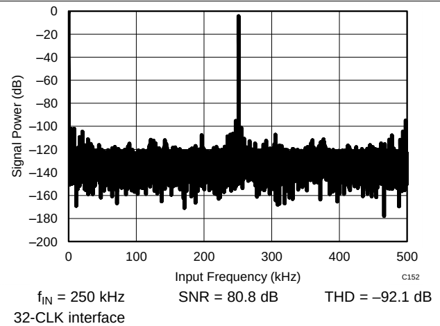
Figure 27. Typical FFT
