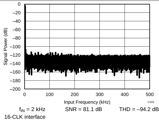
Figure 24. Typical FFT
