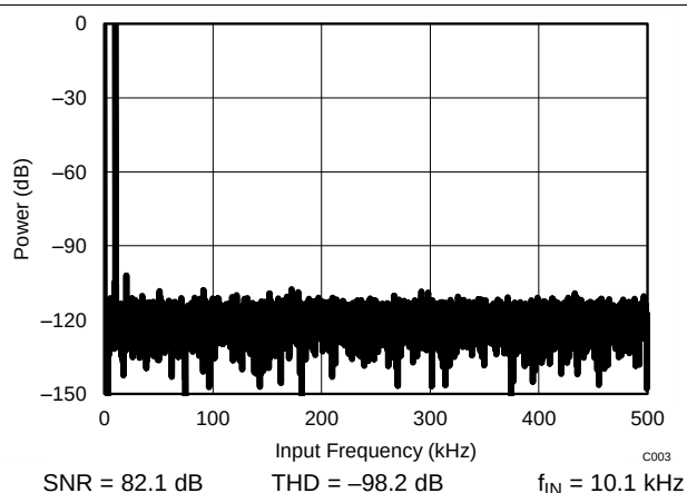
Figure 105. ADS7853 in 32-CLK Interface Mode
