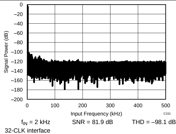
Figure 26. Typical FFT
