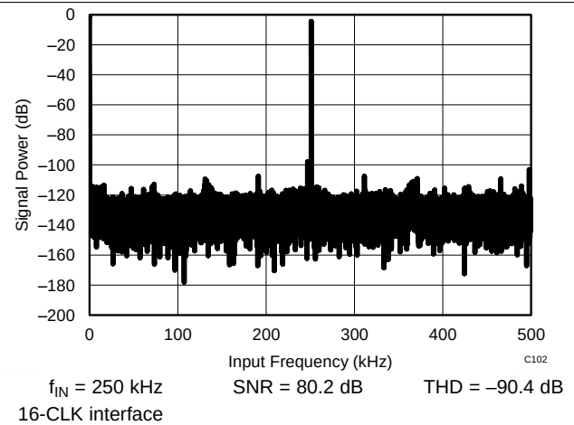
Figure 25. Typical FFT
