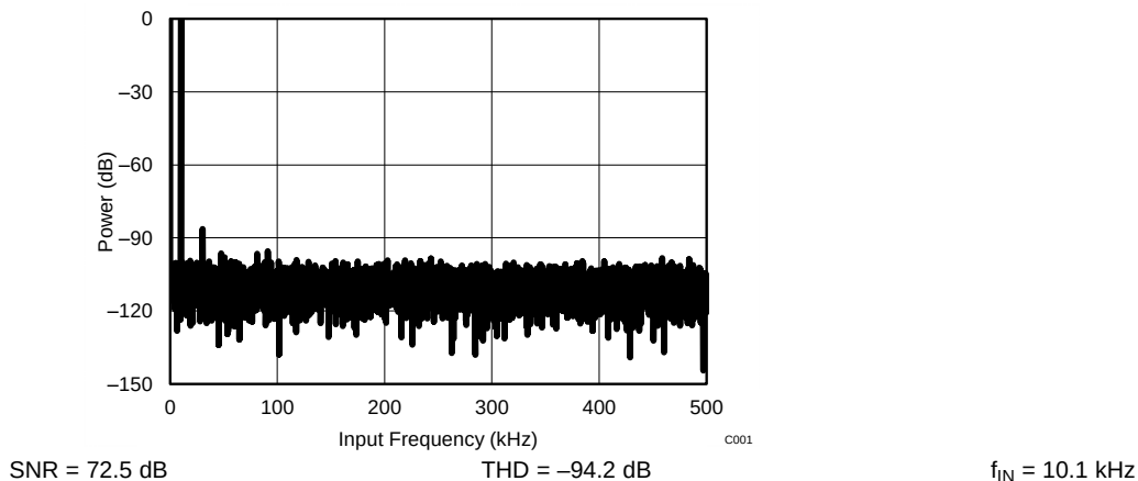
Figure 106. ADS7253 in 32-CLK Interface Mode
