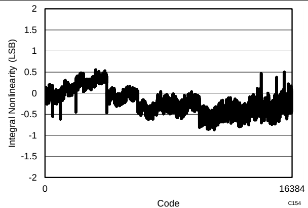
Figure 45. Typical INL
