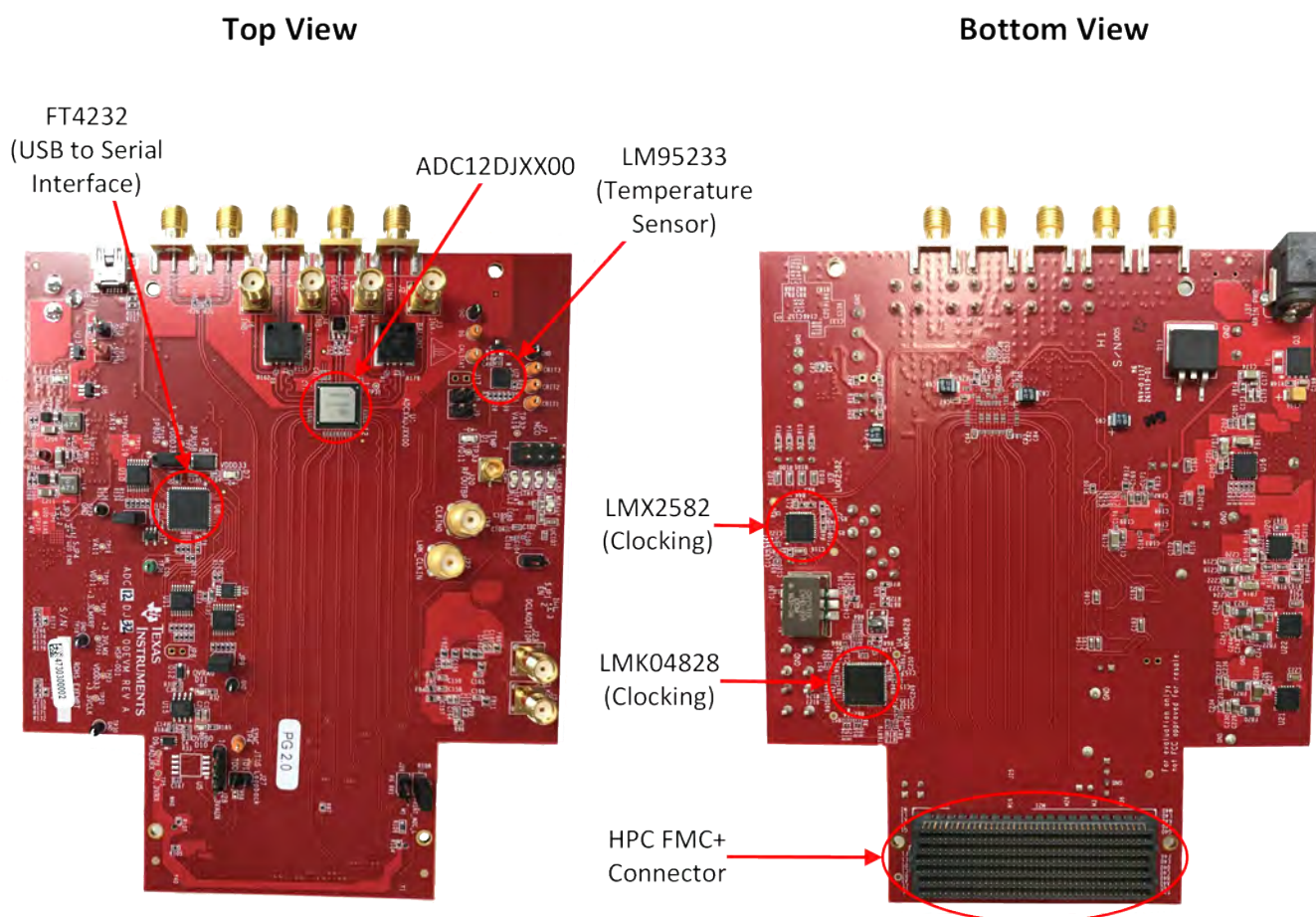
Figure 1-1. EVM Orientation
