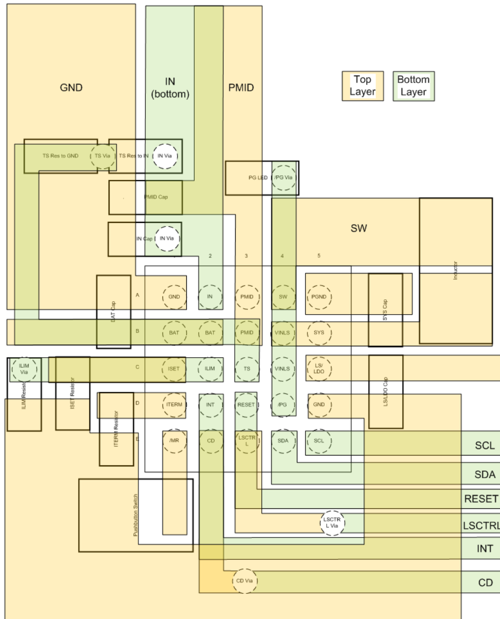
Figure 103. BQ25125 Layout
