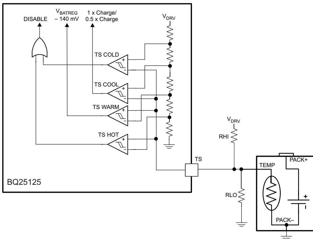
Figure 18. TS Circuit
