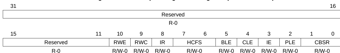
Figure 30-3. HC Operating Mode Register (HCCONTROL)
