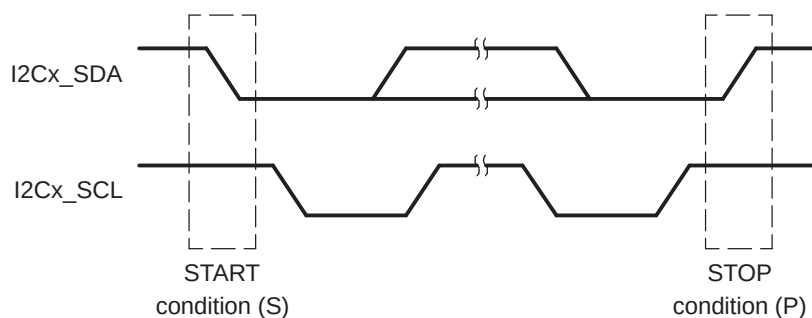
Figure 22-6. I2C Peripheral START and STOP Conditions
