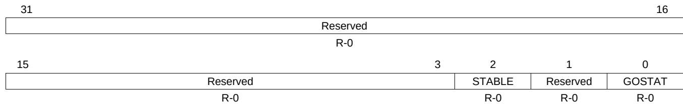
Figure 7-18. PLL Controller Status Register (PLLSTAT)
