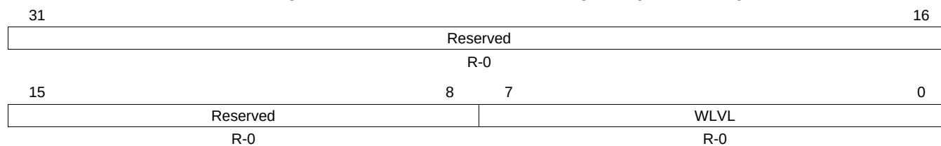
Figure 24-79. Write FIFO Status Register (WFIFOSTS)
