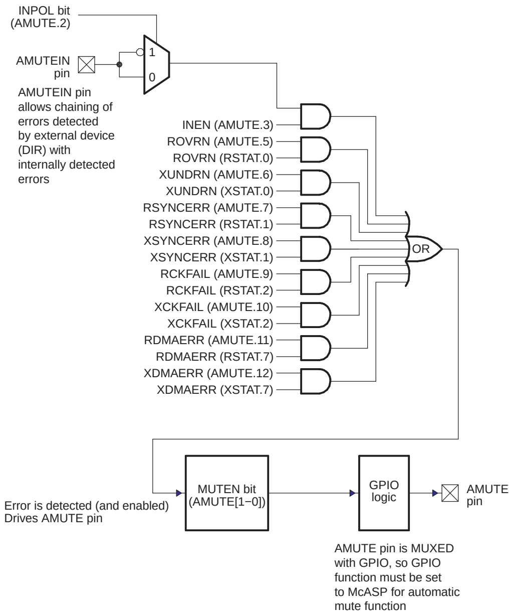
Figure 24-31. Audio Mute (AMUTE) Block Diagram
