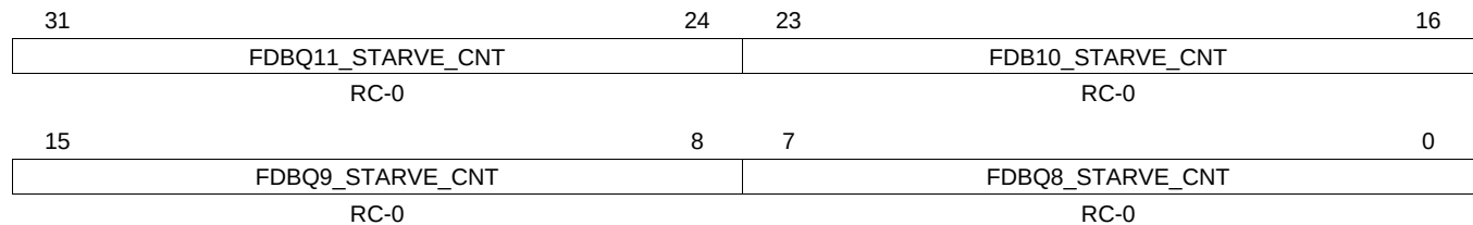
Figure 31-105. Queue Manager Free Descriptor/Buffer Starvation Count Register 2 (FDBSC2)
