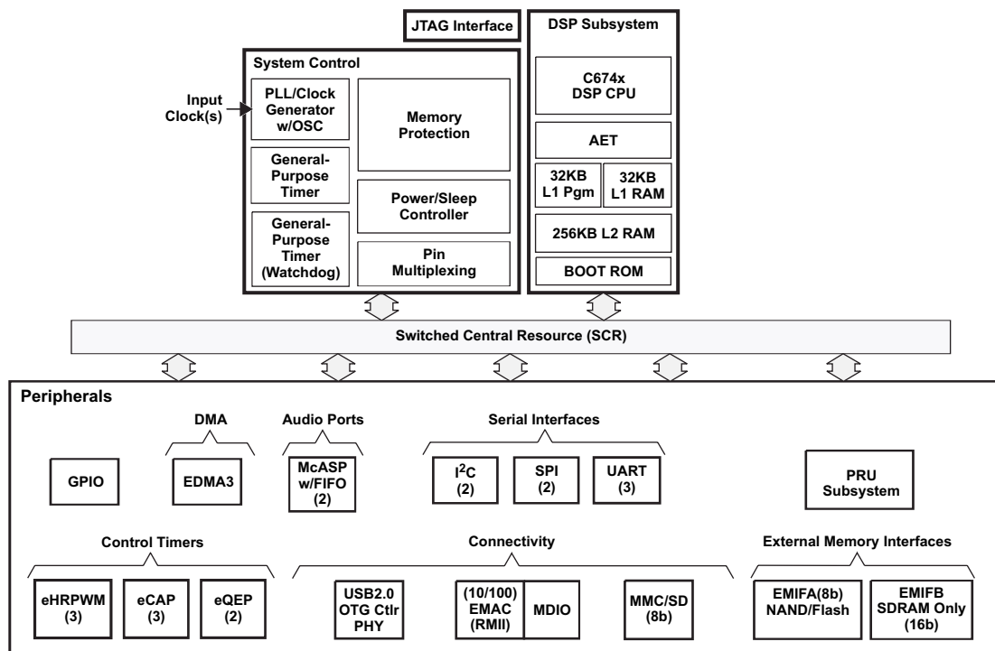
TMS320C6745 DSP Block Diagram
