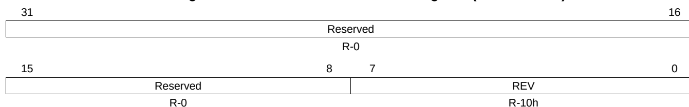
Figure 30-2. OHCI Revision Number Register (HCREVISION)
