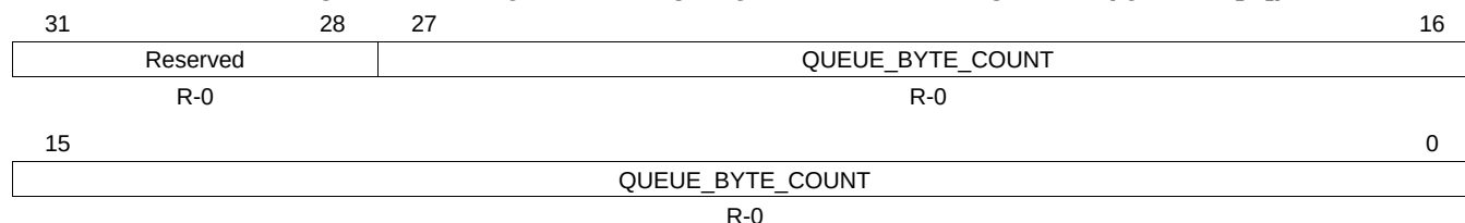
Figure 31-116. Queue Manager Queue N Status Register B (QSTATB[N])
