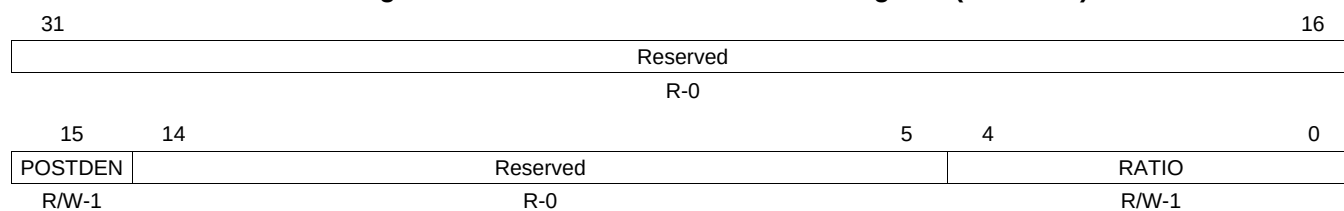
Figure 7-16. PLL Post-Divider Control Register (POSTDIV)
