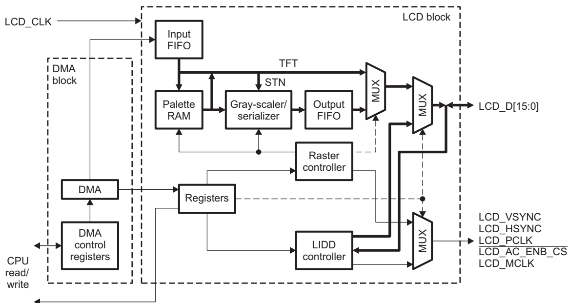
Figure 23-1. LCD Controller
