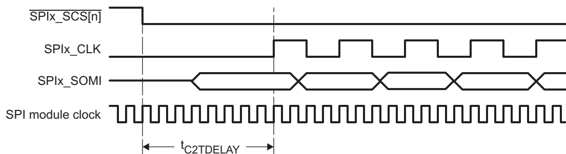
Figure 27-34. Example: t_{\text{C2EDELAY}} = 8 SPI Module Clock Cycles
