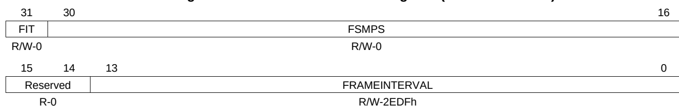
Figure 30-15. HC Frame Interval Register (HCFMINTERVAL)
