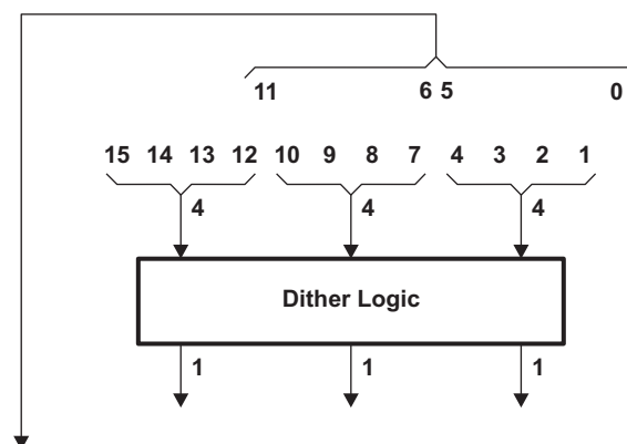
Figure 23-29. 16-BPP STN Mode
