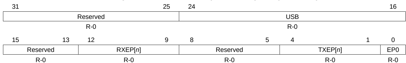
Figure 31-38. USB Interrupt Mask Register (INTMSKR)
