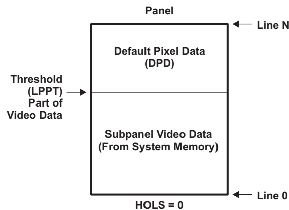
Figure 23-40. Subpanel Display: SPEN = 1, HOLDS = 0
