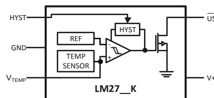
Figure 2. LM27-__K
