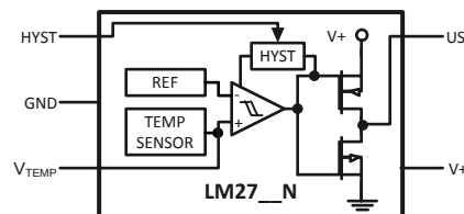
Figure 4. LM27-__N
