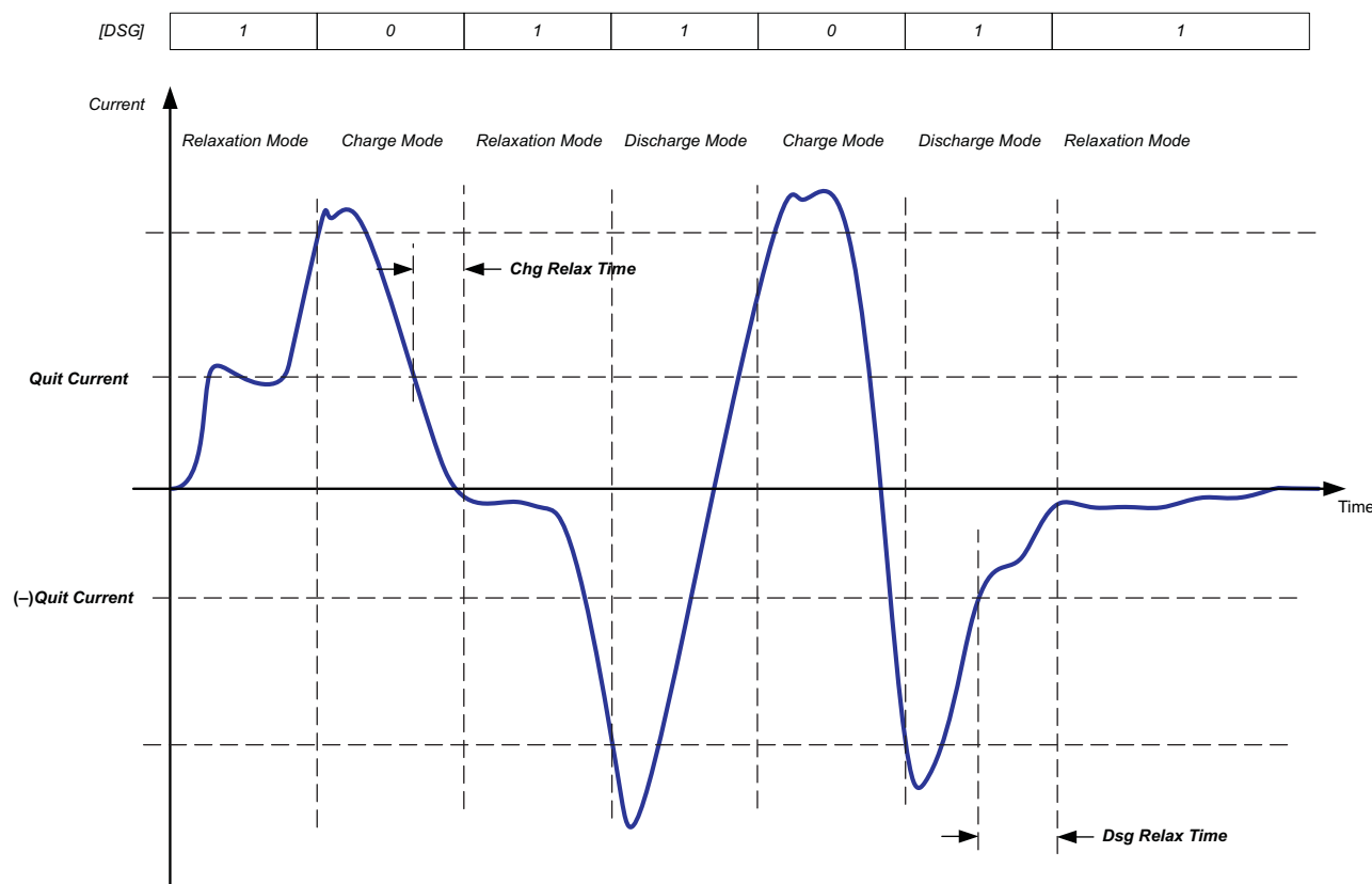
Figure 1-3. Fuel Gauge Operating Mode Example
