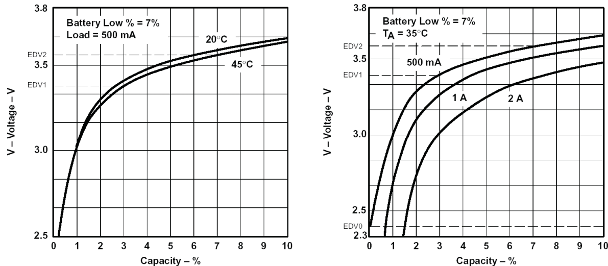
Figure 1-2. (a) EDV Calculations vs Capacity for Various Temperatures, (b) EDV Calculations vs Capacity for Various Loads
