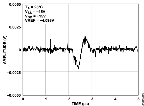
Figure 12. Digital Crosstalk
