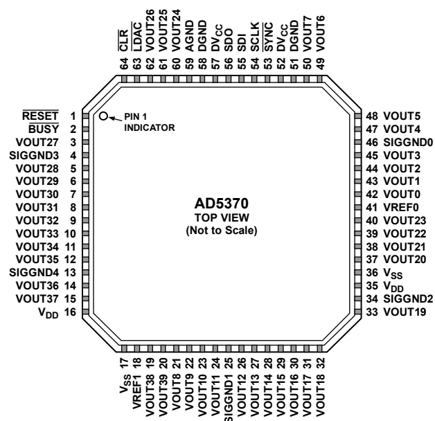
Figure 6. 64-Lead LFCSP Pin Configuration
