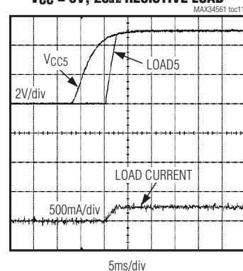
TURN-ON WAVEFORMS V CC = 5V, 20 \Omega RESISTIVE LOAD
