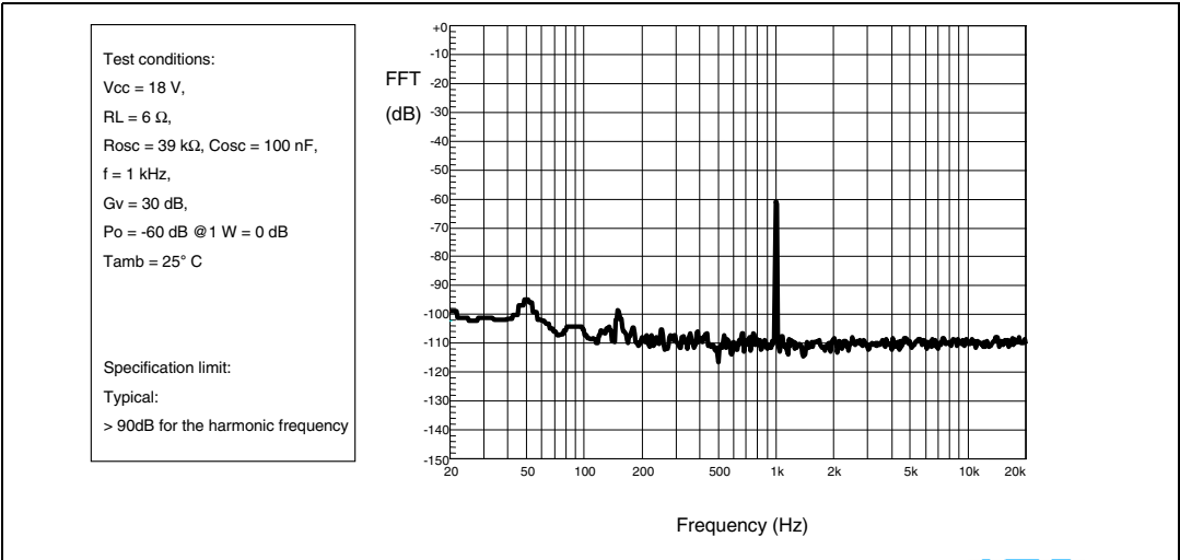
Figure 10. FFT -60 dB
