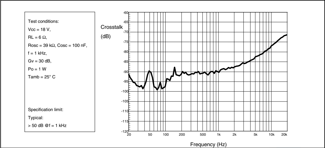
Figure 8. Crosstalk vs frequency
