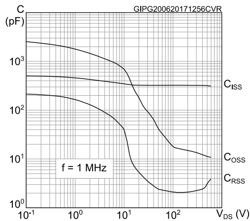
Figure 8: Capacitance variations
