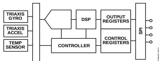
Figure 12. Basic Operation
