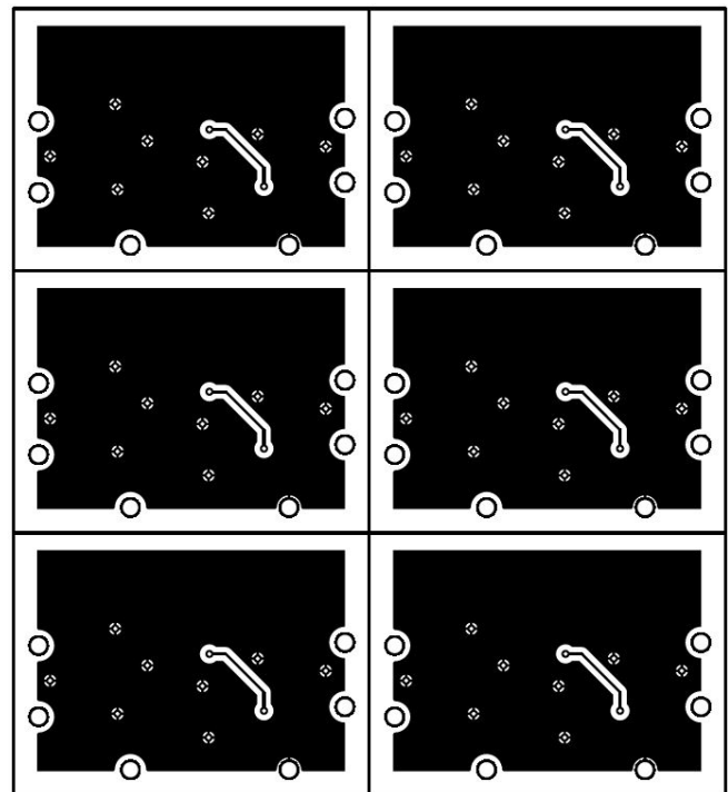
Figure 5. INA210-215EVM Bottom Layer
