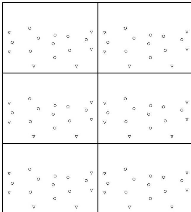
Figure 7. INA210-215EVM Drill Drawing
