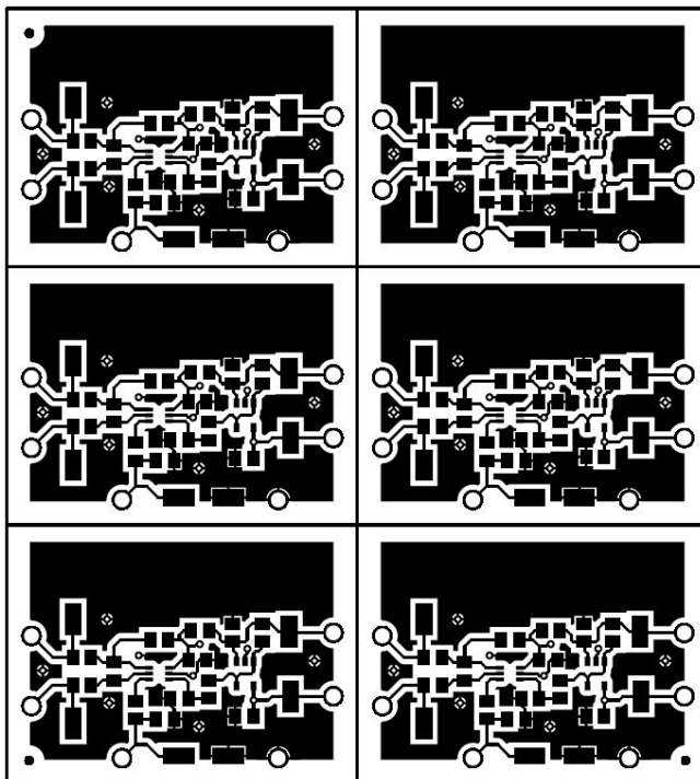
Figure 4. INA210-215EVM Top Layer
