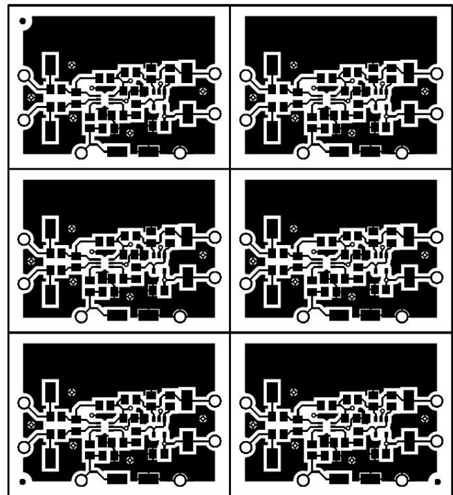
Figure 3. INA210-215EVM Top Solder Mask
