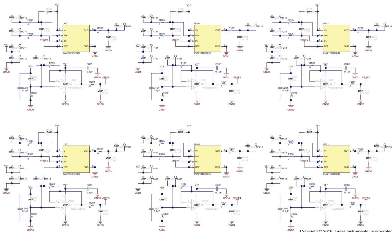
Figure 1. INA210-215EVM Schematic
