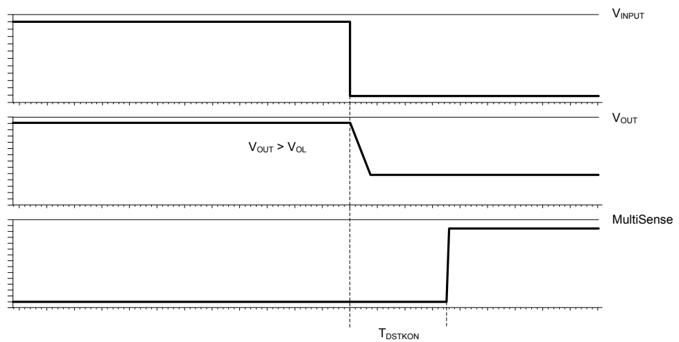
Figure 8. T_{\text{DSTKON}}
