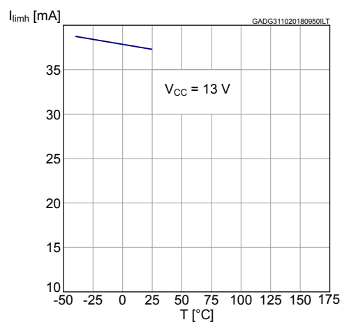
Figure 30. I_{limH} vs. T_{case}
