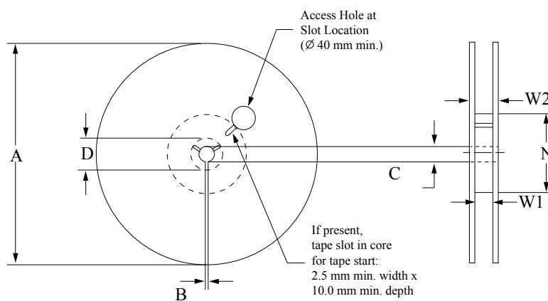
Figure 49. PowerSSO-16 reel 13"
