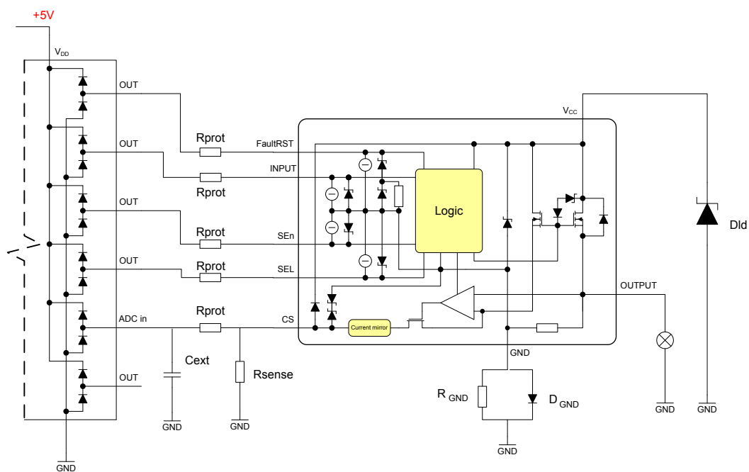
Figure 34. Application diagram
