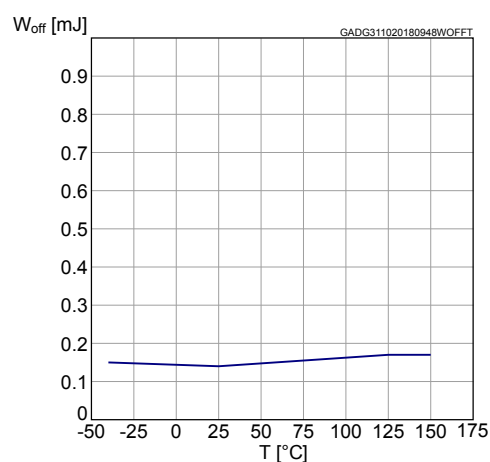
Figure 29. W_{off} vs. T_{case}
