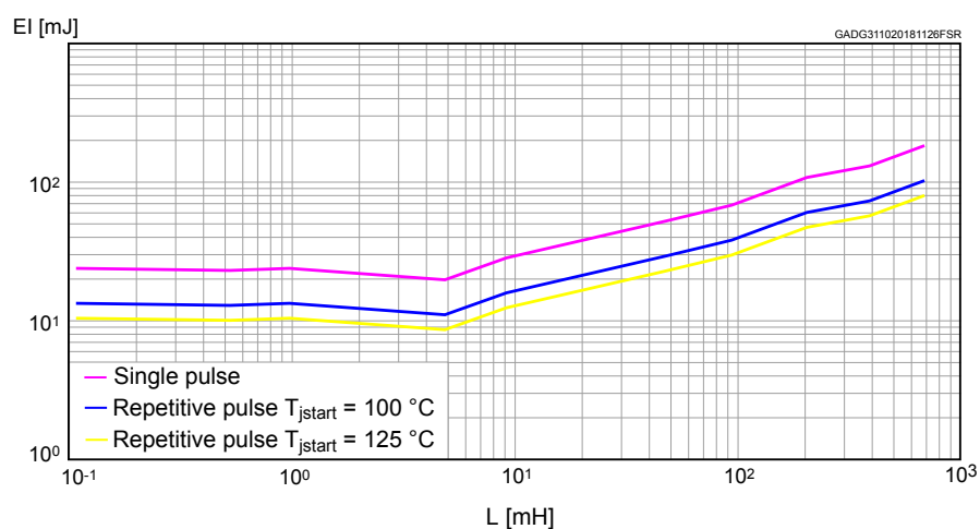
Figure 42. Maximum turn off energy versus inductance
