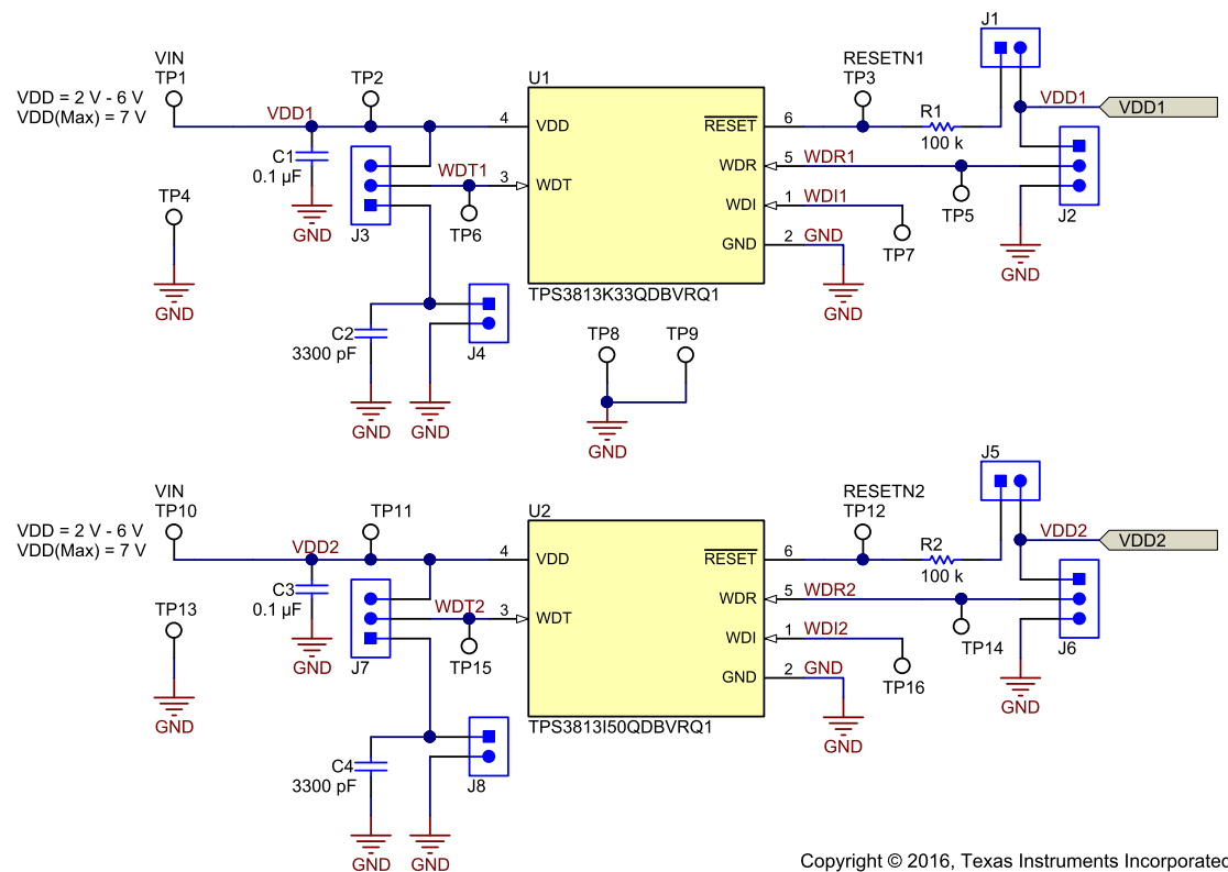
Figure 2. TPS3813xxxQ1EVM Schematic
