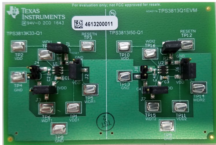
Figure 1. TPS3813xxxQ1EVM Board
