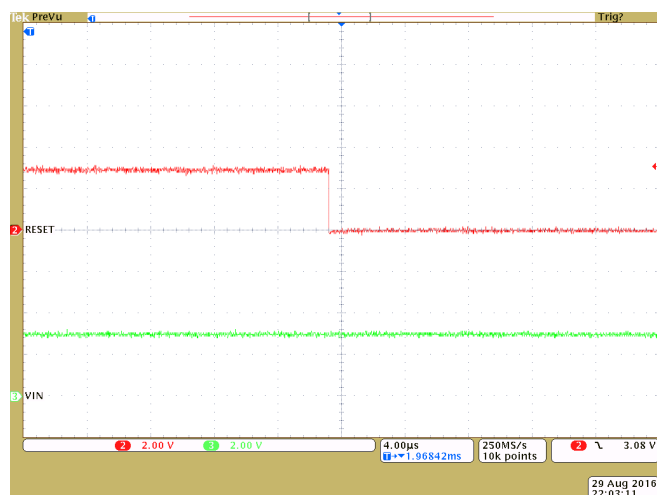
Figure 13. Fall Time TPS3813K33-Q1
