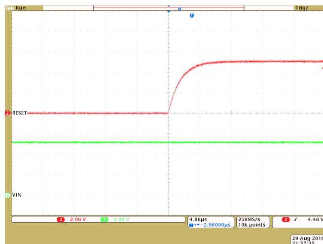
Figure 12. Rise Time TPS3813I50-Q1
