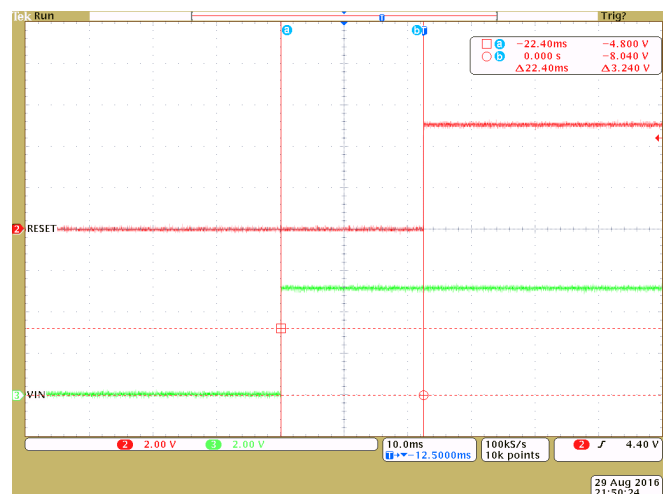
Figure 10. Delay Time TPS3813I50-Q1
