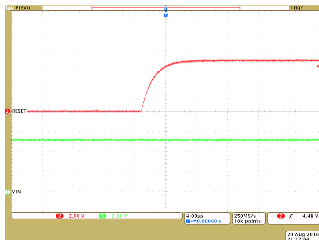
Figure 11. Rise Time TPS3813K33-Q1
