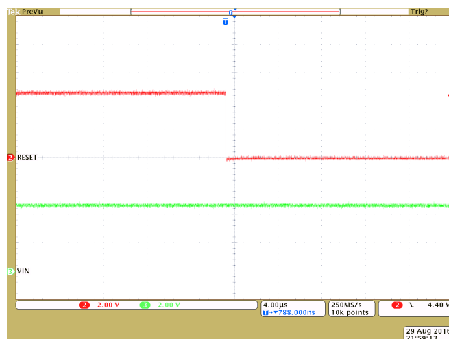
Figure 14. Fall Time TPS3813I50-Q1
