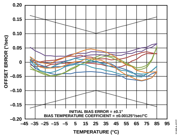
Figure 9. Offset (Bias) Error vs. Temperature, -40^\circ\text{C} to +85^\circ\text{C} to -40^\circ\text{C}
