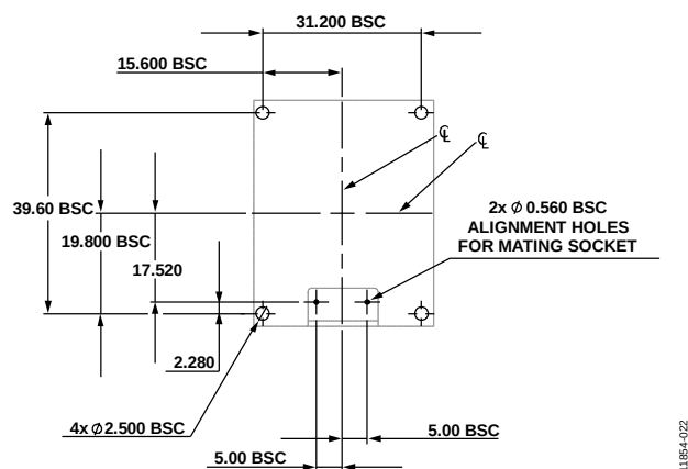
Figure 24. Suggested Mounting Hole Locations, Connector Down
