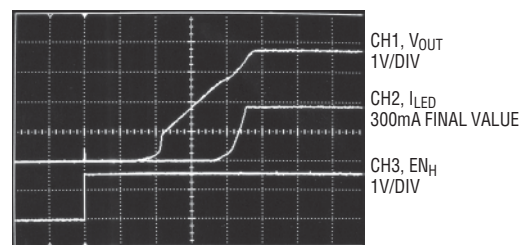
Start-Up Transient
