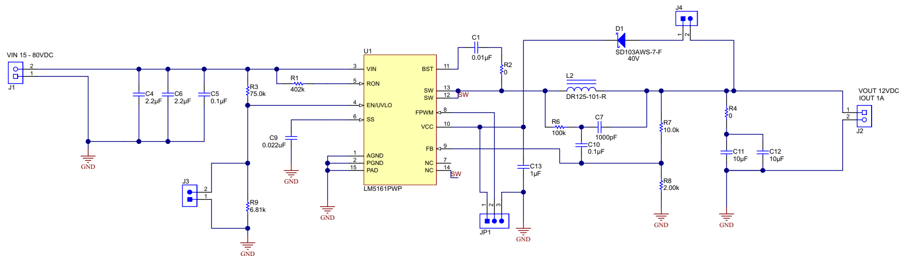
Figure 25. Synchronous Buck Application Circuit
